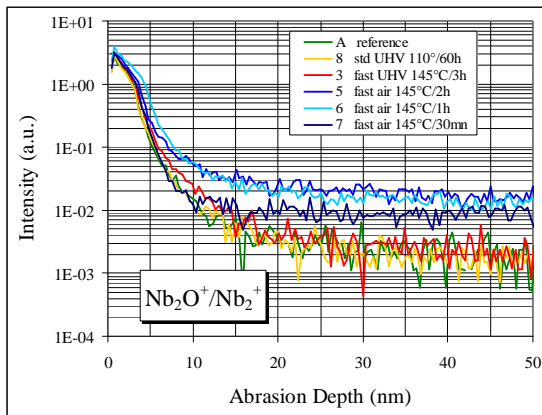
Figure 5: TOF-SIMS profiles of \text{Nb}_2\text{O} / \text{Nb}_2
