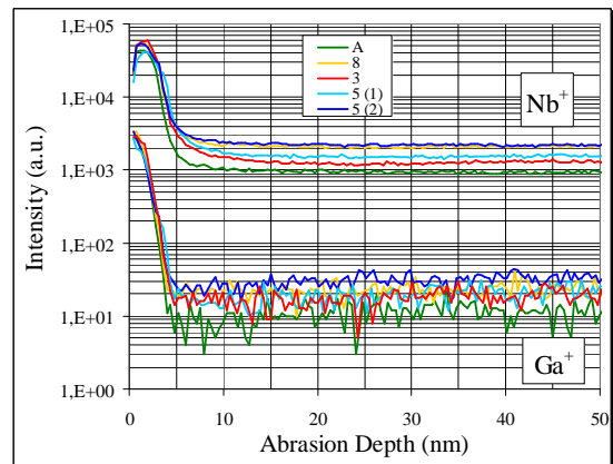
Figure 4: TOF-SIMS profiles of Nb and implanted Gallium ions (coming from the analysis beam).
