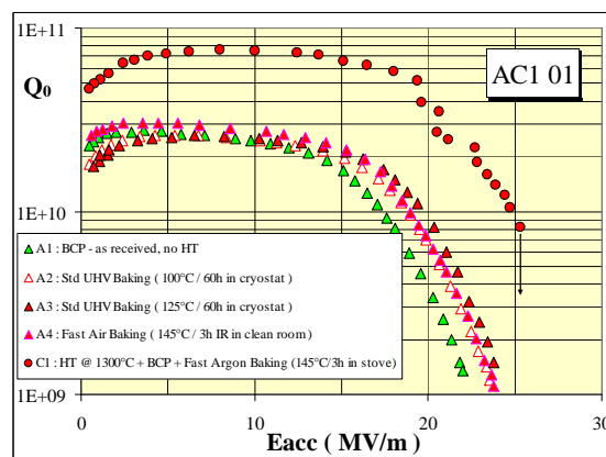
Figure 7: No Baking effect on Q-slopes for AC1-01.
