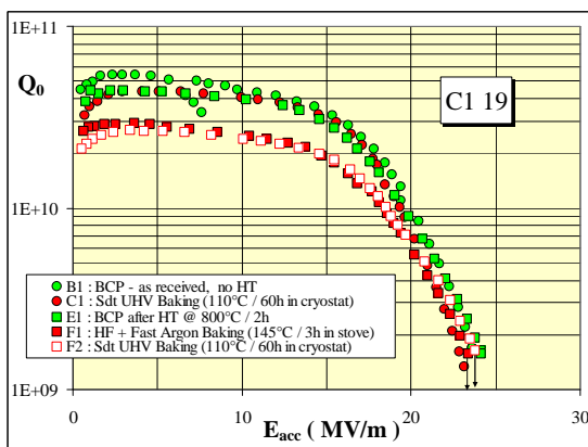
Figure 6: Q-slope unchanged after baking on C119
