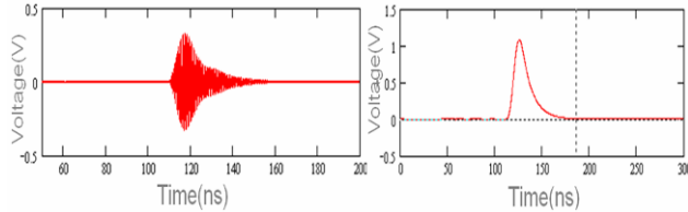
Figure 5: RF (a) and IF (b) signals from the \Delta channel.
