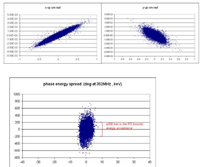
Figure 7 Beam phase space at the exit of the SCL: transverse planes (top) and longitudinal plane (bottom).
