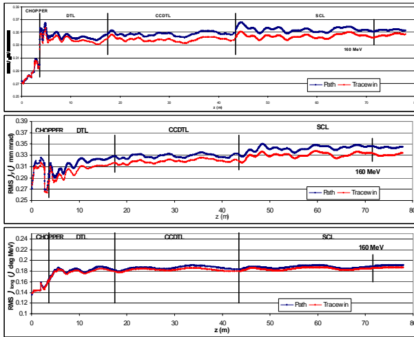
Figure 9 Rms emittance from 3 to 160 MeV. From top to bottom: x-px; y-yp and longitudinal.
