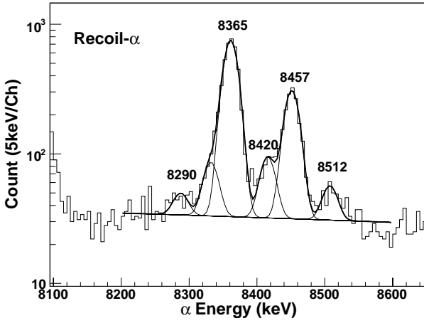
Fig. 4. Portion of the \alpha decay spectrum, resulting from recoil- \alpha correlations, in the ^{255}\text{Lr} region. Data are taken from the JYFL experiment.
