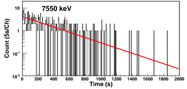
Fig. 8. Upper panel: alpha-decay spectrum of ^{251}\text{Md} resulting from recoil- \alpha - \alpha correlations. Lower panel: time distribution for the 7550 keV \alpha decay. Data are taken from the JYFL experiment.
