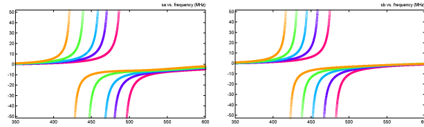
Figure 4. s fit vs. frequency (350 to 600 MHz) for segment ca_x ; End 1 at left: rod lengths 135, 140, 144, 150 and 155 mm (right to left). End 2 at right: rod lengths 135, 140, 145, 150 and 155 mm (right to left).
