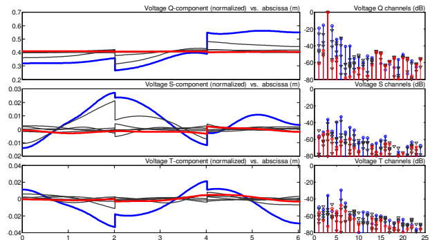
Figure 9. Left: Q, S and T components of accelerating mode Q_{0+0+0} vs. abscissa; blue: un-tuned, red: tuned, black: intermediate steps. Curves are normalized according to \int V_Q^2 dz = 1 . Right: spectral coefficients of Q, S and T components (dB) vs. mode index.
