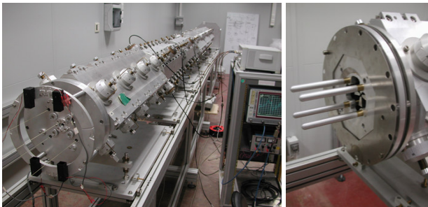
Figure 1 left: cold model with test bench Right: coupling cell with dipolar rods and 0.8mm shims on either side
