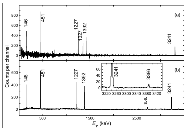
FIGURE 6. The upper panel (a) shows the energy projection of the two dimensional matrix of ^{54}\text{Ni} for the range 0.05 \mu\text{s} \leq t \leq 1.0 \mu\text{s} . In the lower panel (b), the \gamma\gamma coincidence with one of the transitions at 451, 1227 and 1392 keV demonstrates the correlation to other observed lines.
