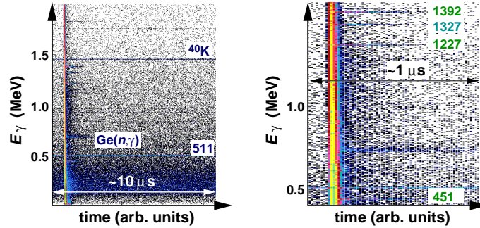
FIGURE 5. ^{54}\text{Ni} gated two dimensional matrices of \gamma -energy versus time after implantation.
