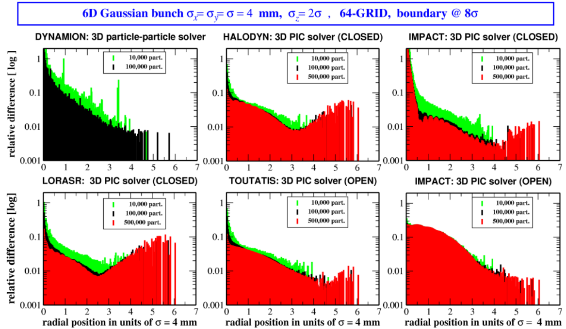
Figure 2 error \delta E/E for DYNAMION and PIC codes with a grid resolution of 64^3 ( 65^3 ).
