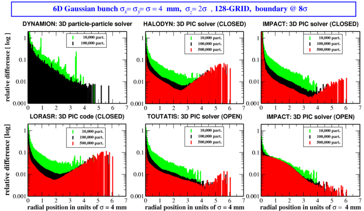
Figure 3 Field error \delta E/E for DYNAMION and PIC codes with a grid resolution of 128^3 ( 129^3 )
