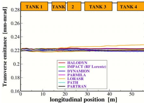
Figure 17 RMS transverse emittance computed by all the codes and plotted along the DTL.
