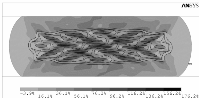
Fig. 6. Total strain in the x direction of the ALSTOM/CEA Nb_3Sn internal tin wire after a 48% reduction in diameter.
