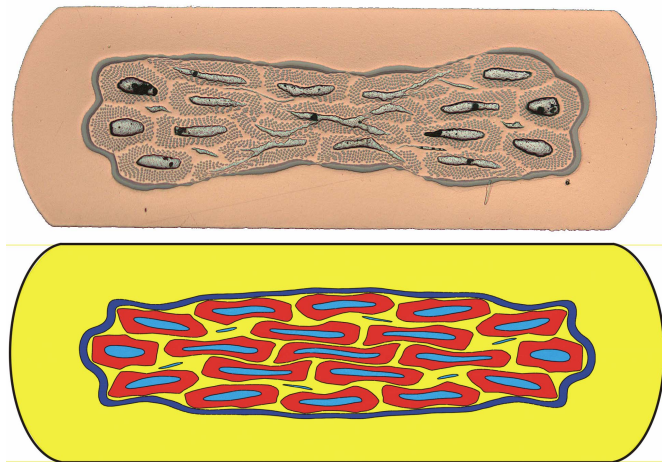
Fig. 5. ALSTOM/CEA Nb_3Sn internal tin wire after a 48% reduction in diameter. The observed deformation is shown together with the FE analysis result.
