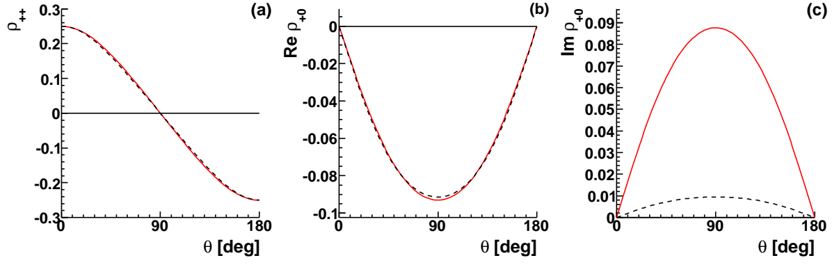
FIG. 2: Angular dependence of the elements of the \rho density matrix: \rho_{++}(\lambda) (a), \text{Re}\rho_{+0}(\lambda) (b), \text{Im}\rho_{+0}(\lambda) (c). The full line corresponds to a 10% width, the dashed line to 1% width.
