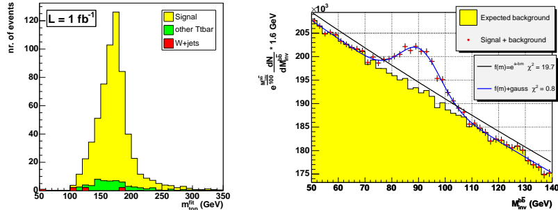
Fig. 9. Left : expected (jjb) mass distribution in semi-leptonic t\bar{t} decays [12]. Right : Z \rightarrow b\bar{b} resonance above the QCD background, in three-jet events [13].
