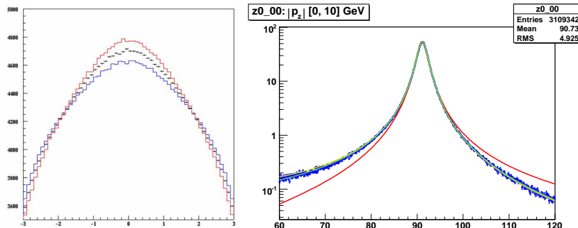
Fig. 3. Left : two extreme predictions of the Z rapidity distribution (histograms), and example pseudo-data (dots) corresponding to 10 \text{ fb}^{-1} . Right : the dilepton mass distributions, as seen in data (histogram), and according to various models. The symmetric curve is a pure Breit-Wigner, the first tilted curve includes final state radiation effects, and the second tilted curve includes structure function effects.
