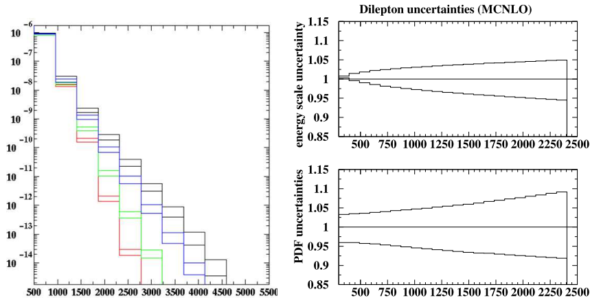
Fig. 1. Left : dijet cross-section uncertainty bands in the Standard Model (upper pair of curves), and in the presence of extra dimensions of compactification scale 6, 4 and 2 TeV (pairs from top to bottom). Right : dilepton production uncertainty bands, arising from the NLO scale dependence (top), and from structure functions (bottom).
