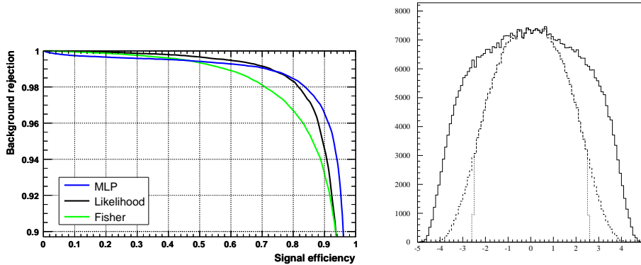
Fig. 4. Left : performance of electron identification in the ATLAS forward calorimeter [6]. Right : Z rapidity acceptance when both electrons have |\eta| < 2.5 (inner histogram); when one electron has |\eta| < 2.5 , and the other has |\eta| < 5 (intermediate histogram); and the full distribution (outer histogram).
