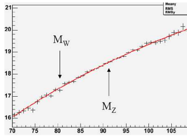
Fig. 8. Average value of p_T(l) , measured in Drell-Yan events, as a function of the lepton pair invariant mass. Both axes are labeled in GeV.
