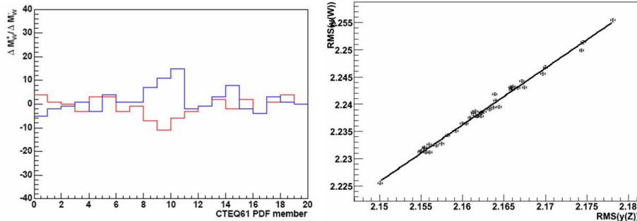
Fig. 6. Left : bias on m_W induced by a \pm 1\sigma variation of each of the 20 parameters defining the CTEQ6 PDF's. Right : correlation between the W and Z rapidity distributions, when varying the proton structure functions within uncertainties. A similar correlation is observed for the W and Z p_T distributions.
