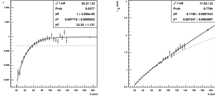
Fig. 7. Measurement of scale (left) and resolution (right) as a function of the lepton energy, in Z boson decays [9].
