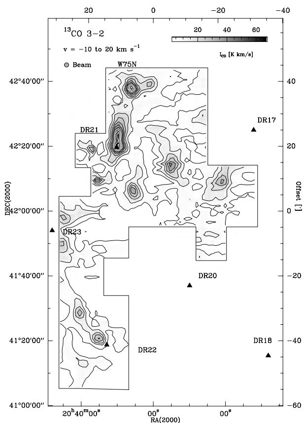
Fig. A.1. Line-integrated ( v=-10 to 20 km s ^{-1} ) ^{13}\text{CO} 3 \rightarrow 2 emission from the CygX-North region as observed with KOSMA. Contour lines are drawn in black from 3\sigma to 57\sigma in steps of 9\sigma and in white from 60\sigma to 87\sigma in steps of 9\sigma with 3\sigma=2.3 K s ^{-1} .
