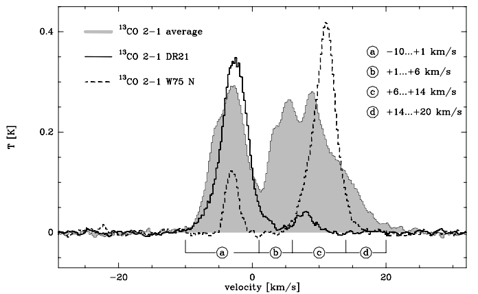
Fig. 4. The spatially-averaged spectrum of ^{13}\text{CO} 2 \rightarrow 1 emission is displayed in grey. Single ^{13}\text{CO} 2 \rightarrow 1 spectra taken from the DR21 and W75N regions (reduced by a factor of 30 and 20, respectively) are shown as a straight and dashed line. The main velocity ranges with ^{13}\text{CO} emission are indicated and labeled.
