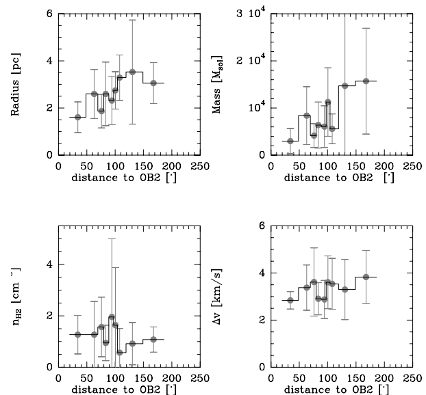
Fig. C.2. Variation in radius, mass, average H 2 -density ( n_{\text{H}_2} ), and line width ( \Delta v ) of the clumps found in the 13 CO Cygnus X survey with distance to the Cyg OB2 cluster. The data are shown in bins of 10, the error bars indicate standard deviation.
