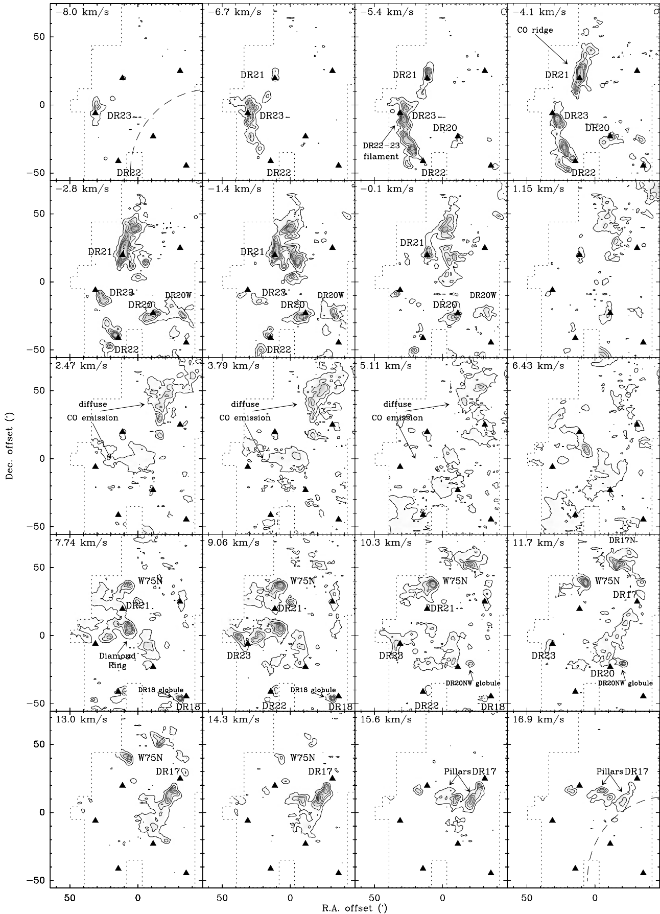
Fig. 3. Channel maps of ^{13}\text{CO} 2 \rightarrow 1 emission with a step size of \sim 1.3 km s ^{-1} in the CygX-North region are shown. The lowest contour is the 6\sigma level and contours go then in 6\sigma steps. Triangles mark the positions of the HII regions DR17 to DR23. These sources are labeled only in the relevant velocity interval. Prominent features (filaments, globules, etc.) mentioned in the text are denoted by arrows. The dashed circle in the first and last channel shows the extent of the OB 2 association.
