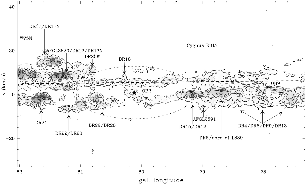
Fig. 10. Position-velocity cut in ^{13}\text{CO} 2 \rightarrow 1 averaged over Galactic latitudes \sim -1^\circ to \sim 2^\circ . Maps of ^{13}\text{CO} emission in the whole Cygnus X region in Galactic coordinates are found in Figs. 7 to 9. The minor axis of the dotted ellipse is defined by the highest and lowest velocities of globules ( 13 \text{ km s}^{-1} and -11 \text{ km s}^{-1} ) symmetrically around +1 \text{ km s}^{-1} . The major axis is given by the diameter of the OB2 cluster ( 2^\circ , Knödelseder et al. 2000). The center is defined by the longitude of the OB2 cluster center ( 80.12^\circ , Knödelseder et al. 2000) and by 1 \text{ km s}^{-1} in velocity space (see above). The dashed line indicated the possible velocity component of the Cygnus Rift, considering a distance of 800 pc and using the Galactic rotation curve.
