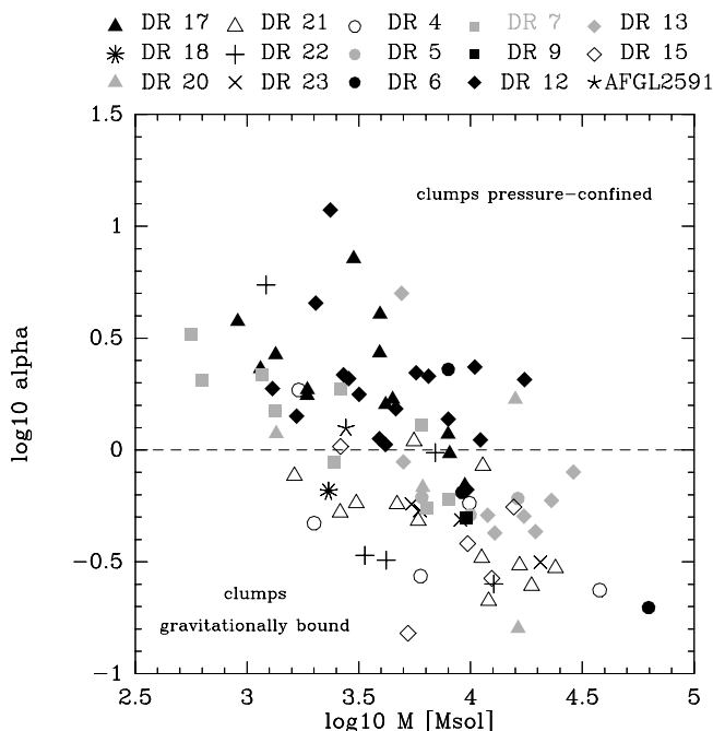
Fig. C.1. Virial parameter \alpha as a function of mass, plotted for the clumps found in Cygnus X. The different symbols allow us to distinguish between clumps of all regions, i.e. DR17–23 in CygX-North and DR4–DR15 and AFGL2591 in CygX-South. Clumps with \log(\alpha) \simeq 0 are in gravitational virial equilibrium.
