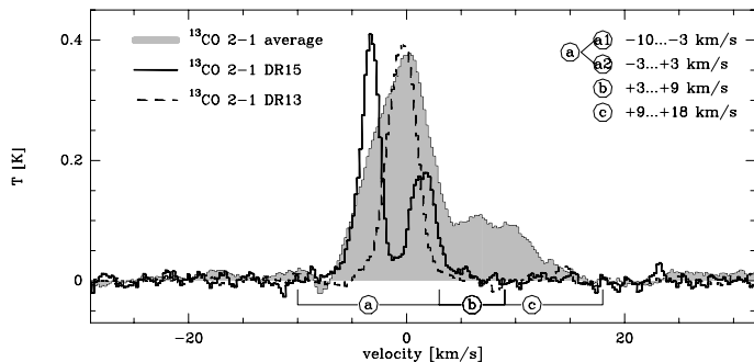
Fig. 6. Spatially-averaged spectrum of ^{13}\text{CO} 2 \rightarrow 1 emission (grey) together with single ^{13}\text{CO} 2 \rightarrow 1 spectra taken from the DR15 and DR13 regions (straight and dashed line, both reduced by a factor of 15). The main velocity ranges with ^{13}\text{CO} emission are indicated and labeled.
