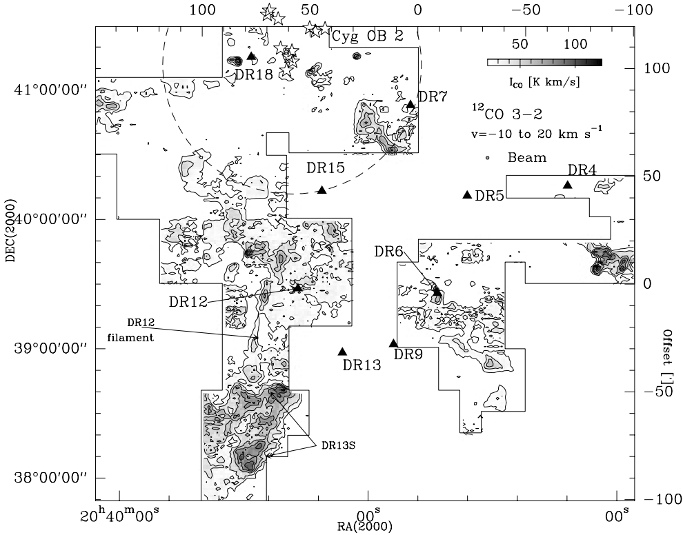
Fig. A.2. Line-integrated ( v=-10 to 20 km s^{-1} ) ^{12}\text{CO} 3 \rightarrow 2 emission from the CygX-South region as observed with KOSMA. Contour lines are drawn in black from 15\sigma to 75\sigma in steps of 12\sigma with 3\sigma=4 K km s^{-1} .
