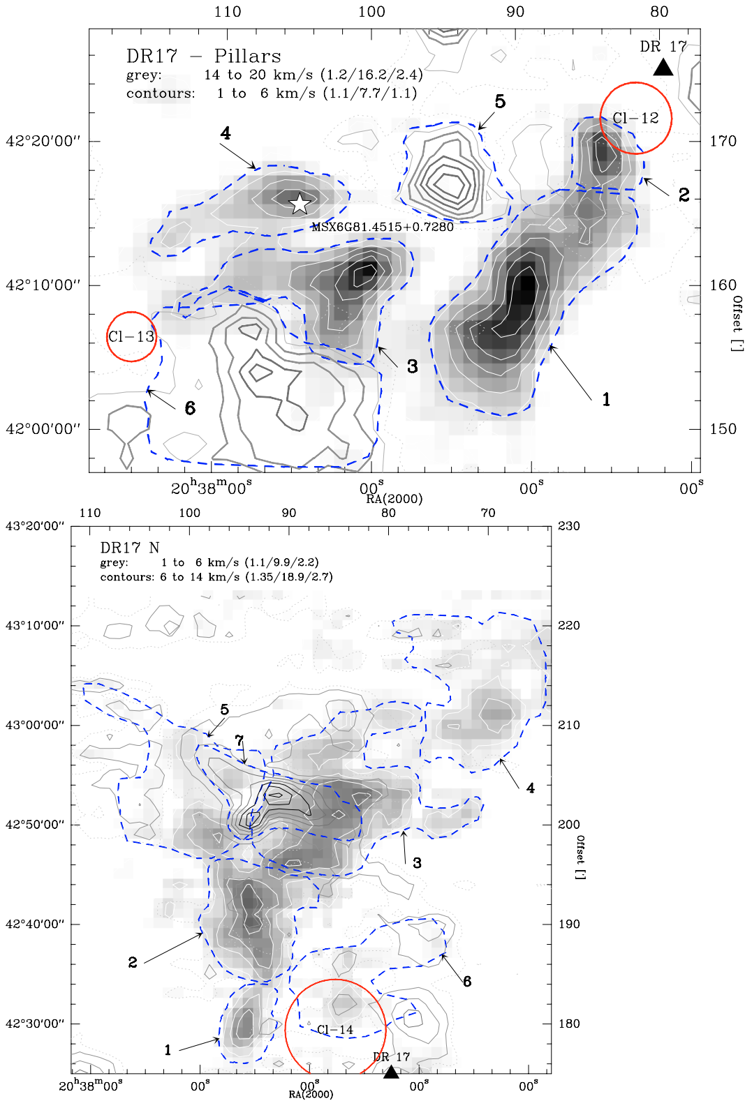
Fig. B.1. Velocity-integrated ^{13}\text{CO} 2 \rightarrow 1 maps of the DR17 and DR17N regions in Cygnus X. Two velocity ranges are shown (one in grey scale and light contours and one with grey to black contours). The level notation is start/end/step with the values in \text{K km s}^{-1} . All contours start at the 3\sigma level. Dashed (blue) contours indicate the 25% maximum intensity level of a clump for the mass determination. Individual clumps are numbered according to Tables C.1 and C.2. Known IR-clusters are indicated by circles (size given by Le Duigou & Knödlseder 2002) and IRAS and MSX sources by stars.
