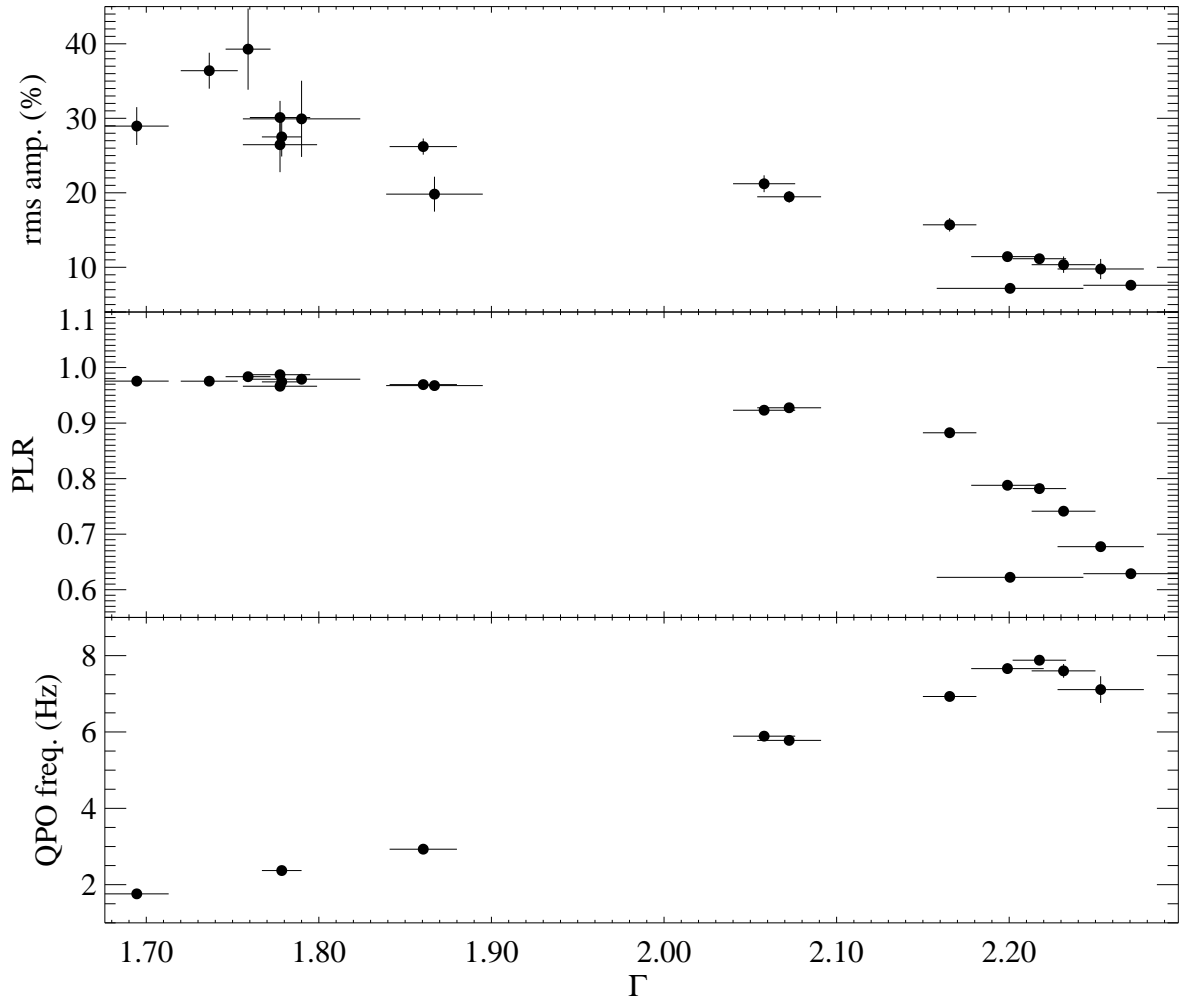
Fig. 4.— The correlation between the photon index and, (a) the rms amplitude of variability, (b) the PLR, and (c) the QPO frequency for observations taken between MJD 52930.9 and MJD 52949.7, excluding the TD-like observation.
