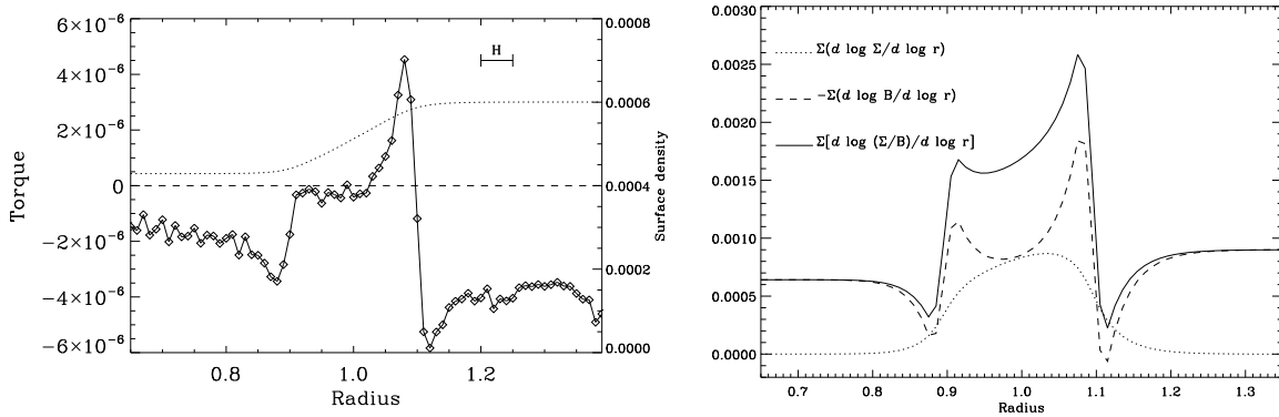
Fig. 4.— Left: surface density profile for the runs of section 4.3 (dotted line and right axis) and total torque exerted by the disk on the planet as a function of its semi-major axis (diamonds and left axis), for a 4 M_{\oplus} planet. Right: Corresponding profiles of the different logarithmic derivatives involved in the expression of the corotation torque, weighted by the surface density, as in Fig. 1.
