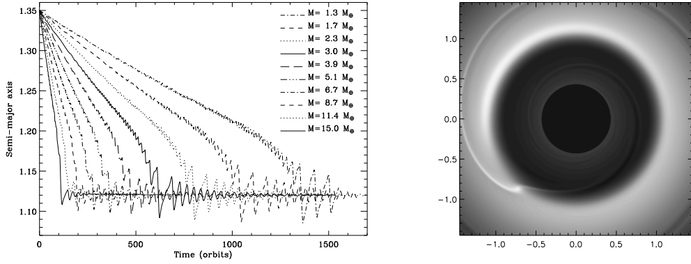
Fig. 3.— Left plot: primary to planet separation curve as a function of time, for the 10 different planet masses. Right plot: snapshot of the surface density map with a 15 M_{\oplus} planet embedded at t = 480 orbits.
