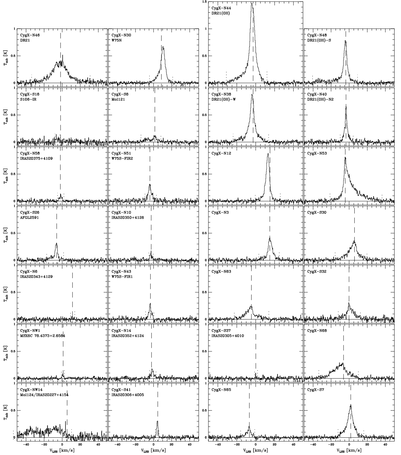
Fig. 5. SiO(2-1) lines observed toward the 28 most massive ( > 40 M_{\odot} ) cloud fragments of Cygnus X: 14 high-luminosity infrared sources on the left and 14 infrared-quiet protostellar cores on the right, both ordered by decreasing M_{1.2 \text{ mm}} from top to bottom. The local velocity at rest of each cloud fragment, as measured by optically-thin tracers, is indicated by a dashed line.
