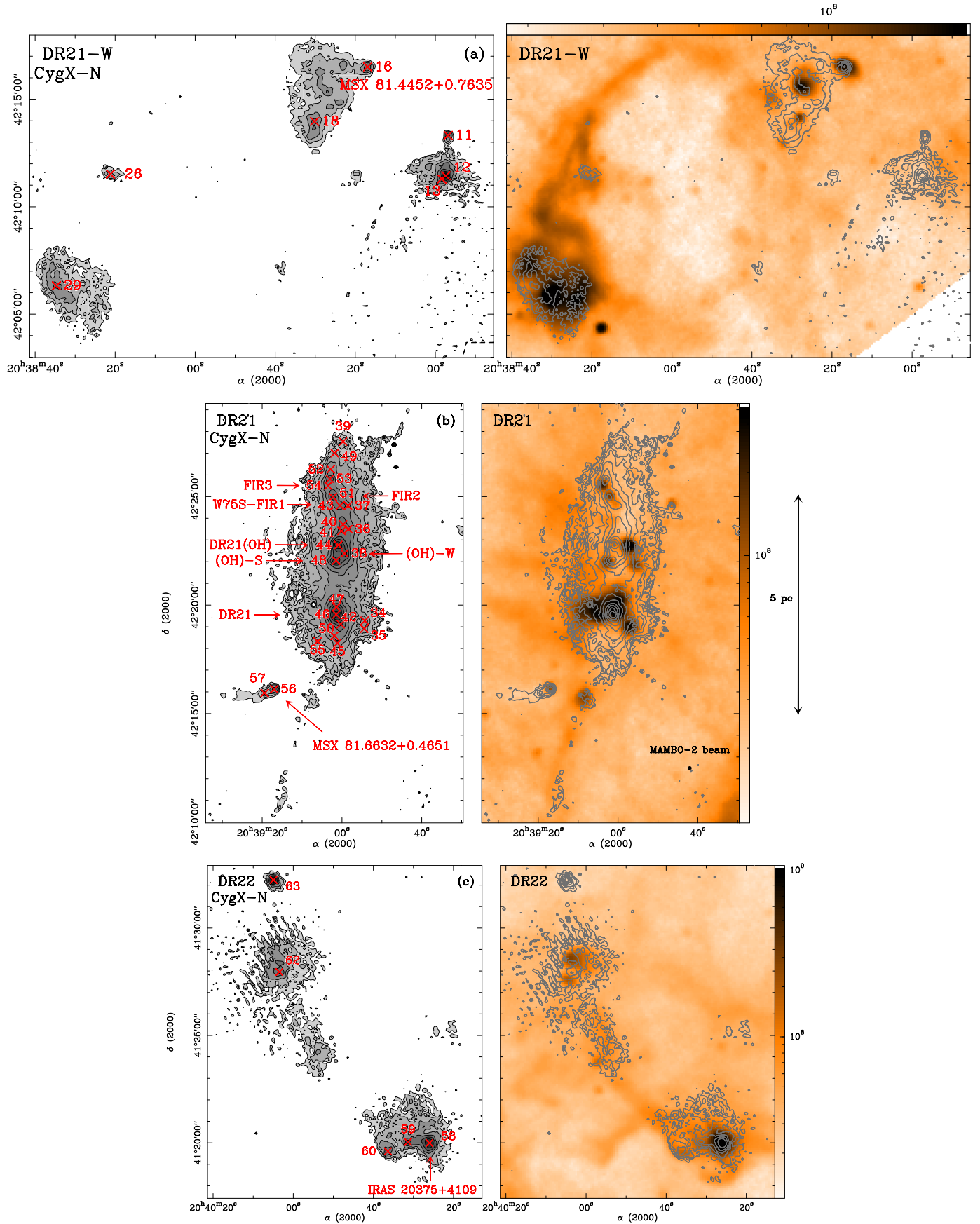
Fig. 3. MAMBO maps of CygX-North ( left : gray-scale and contours, right : contours overlaid on 8\ \mu\text{m} images obtained by MSX and converted to \text{Jy sr}^{-1} ) extracted from Fig. 2a. Regions shown are west of DR21 ( a ), around DR21 ( b ) and DR22 ( c ). The 1.2\ \text{mm} and 8\ \mu\text{m} images have 11'' and 20'' angular resolutions, respectively. The compact cloud fragments discovered in MAMBO images (see Table 1) are labeled and marked by crosses in the gray-scale plot. The infrared sources which coincide with a MAMBO cloud fragment are also indicated. Contour levels are logarithmic and go from 40 to 800\ \text{mJy beam}^{-1} in a and c , and from 40 to 4800\ \text{mJy beam}^{-1} in b .
