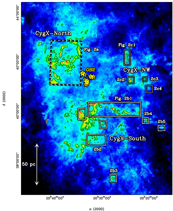
Fig. 1. Extinction map of the Cygnus X complex derived by Bontemps et al. (in prep.) from the stellar reddening of background stars in JHK, using the 2MASS database and a pixel size of 1.3'' . The high-extinction regions are yellow and outlined by the 15 mag contour level. The three molecular cloud ensembles identified by Schneider et al. (2006) are labeled and the nearby Cygnus OB2 association is indicated. The fields mapped with MAMBO or MAMBO-2 are schematically outlined and add up to \sim 3''^2 .
