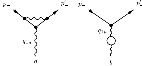
Fig. 2: Some one-loop FD for virtual Compton scattering.
