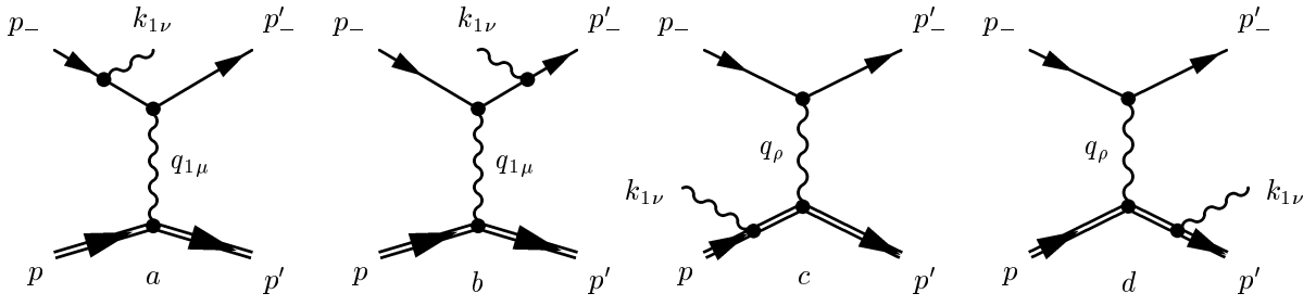
Fig. 1: Born Feynman diagrams for virtual Compton scattering.
