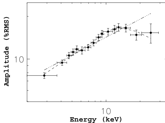
FIG. 6.— Spectrum of the LFGPO from the unique RXTE observation that was simultaneous to INTEGRAL Obs. 4 and the RT. The best model obtained from fits with power law and power law with an exponential cut-off are respectively over-plotted as a dash-dotted and a dashed line. A better fit is obtained with the power law with cut-off.
