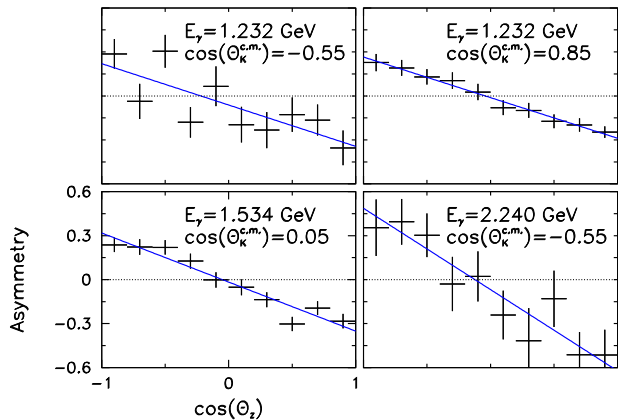
FIG. 2: (Color online) Representative hyperon yield asymmetries as a function of proton decay angle for the case of the C_z observable for the \Lambda . The scales are the same in all plots.
