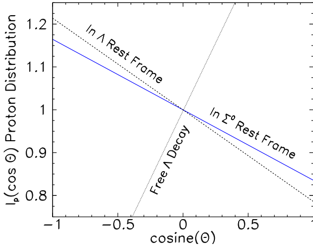
FIG. 18: (Color online) The solid (blue) line shows the proton angular distribution in the \Sigma^0 rest frame, where \theta is the polar angle with respect to the polarization axis \hat{z} . The dashed (black) line shows the expected slope of the proton distribution in the \Lambda rest frame, where the angle \theta in the graph is construed as the proton angle \theta_p , i.e. measured from the axis of the \Lambda 's velocity. The dotted (black) curve shows, for reference, the slope of the proton distribution in the case of fully polarized \Lambda hyperons decaying, where the angle is \theta_p with respect to the \Lambda polarization axis.
