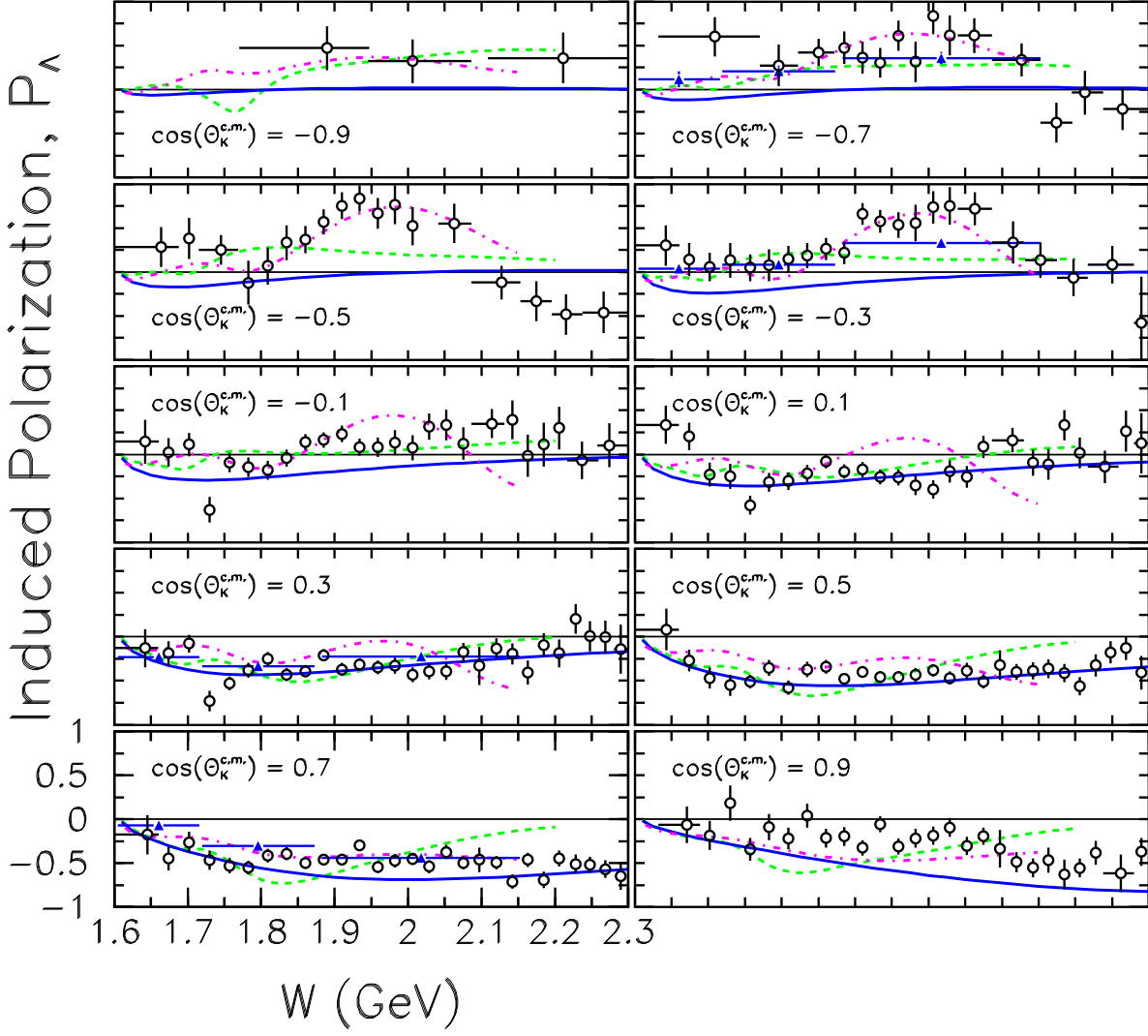
FIG. 11: (Color online) Induced recoil polarization, P , of the \Lambda hyperon in \gamma + p \rightarrow K^+ + \bar{\Lambda} . Open circles (black) from Ref. [4], triangles (blue) from Ref. [2]. The dashed (green) curves are from Kaon-MAID [10], the dot-dashed (magenta) curves are from GENT [12], and the solid (blue) curves are the Regge model GLV [24, 25].
