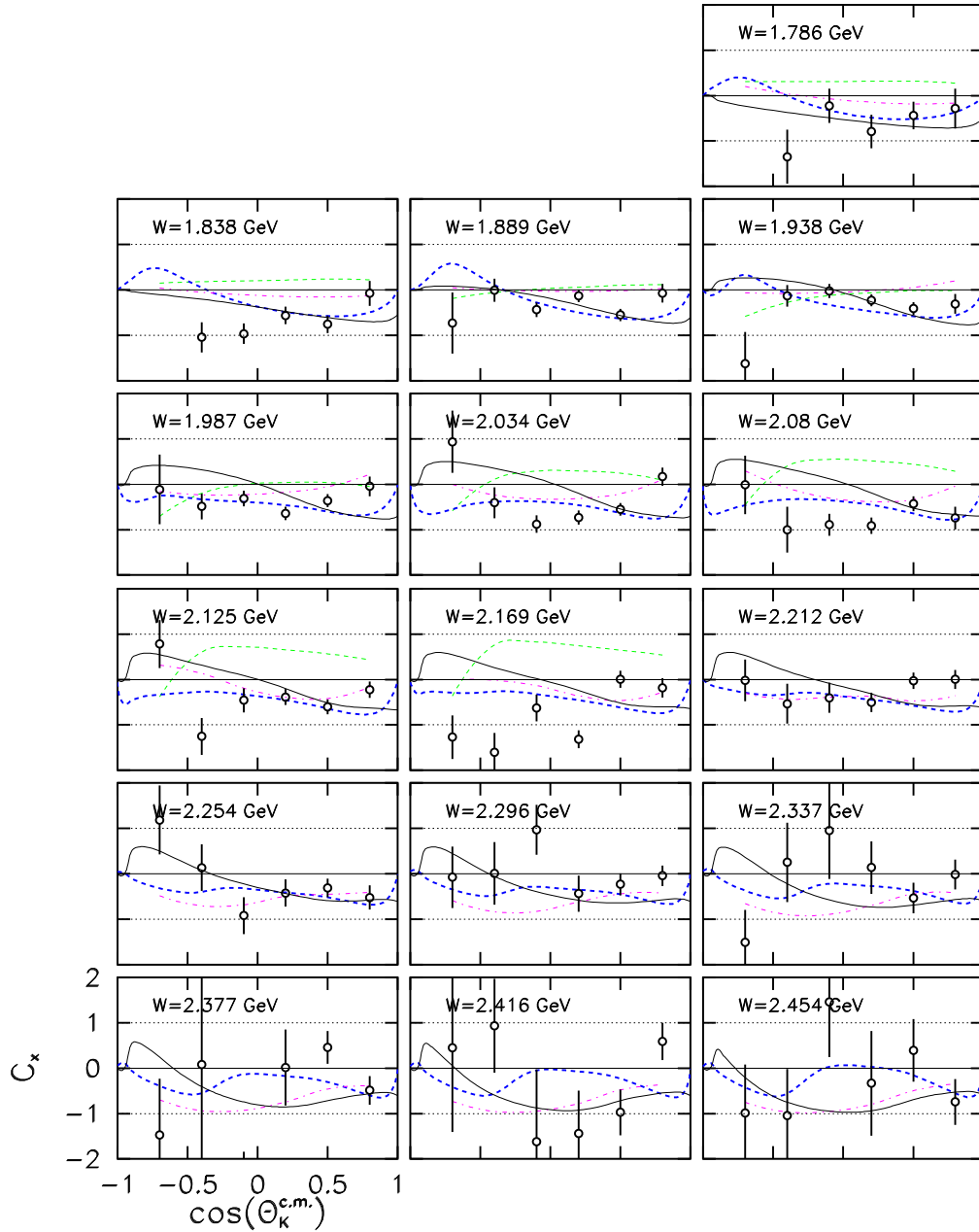
FIG. 16: (Color online) The observable C_x for the reaction \vec{\gamma} + p \rightarrow K^+ + \vec{\Sigma}^0 , plotted as a function of the kaon angle. The 16 panels are for increasing values of W in steps of about 50 MeV. The circles are the results of this measurement, with uncertainties discussed in the text. The thin dashed (green) curves are from Kaon-MAID [10], the thick dashed (blue) curves are from BG [42], the thin solid (black) curves are from RPR [16], and the thick dot-dashed (magenta) curves are from GENT [12].
