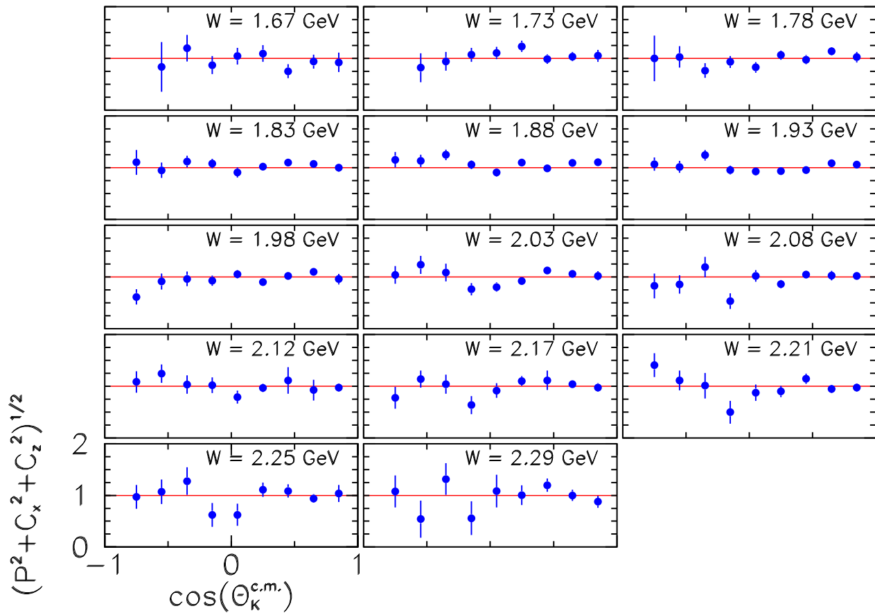
FIG. 10: (Color online) The magnitude of the \Lambda hyperon polarization observable vector R_\Lambda = \sqrt{P^2 + C_x^2 + C_z^2} in the same binning as Figs. 8 and 9. R_\Lambda is consistent with unity over all values of W and kaon angle.
