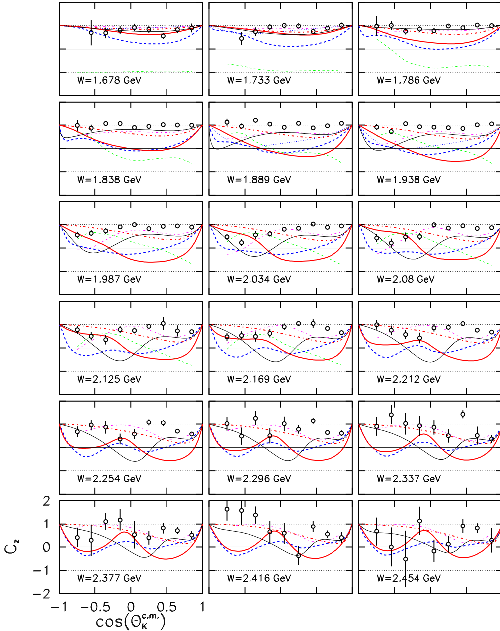
FIG. 8: (Color online) The observable C_z for the reaction \vec{\gamma} + p \rightarrow K^+ + \bar{\Lambda} , plotted as a function of the kaon angle. The 18 panels are for increasing values of W in steps of about 50 MeV. The circles are the results of this measurement, with uncertainties discussed in the text. The thin dashed (green) curves are from Kaon-MAID [10], the thick solid (red) curves are from SAP [18], the thick dashed (blue) curves are from BG [42], the thin solid (black) curves are from RPR [16], and the thick dot-dashed (magenta) curves are from GENT [12]. The thick dot-dashed (red) curves are from GLV [24, 25]. The thin dotted (blue) curves are from SLM [20].
