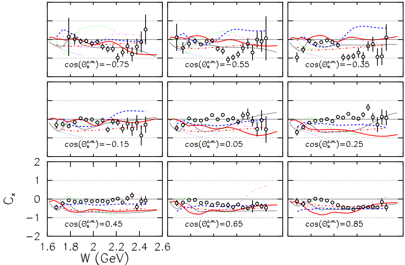
FIG. 7: (Color online) The observable C_x for the reaction \bar{\gamma} + p \rightarrow K^+ + \bar{\Lambda} , plotted as a function of the c.m. energy W . The circles are the results of this measurement, with uncertainties discussed in the text. The thin dashed (green) curves are from Kaon-MAID [10], the thick solid (red) curves are from SAP [18], the thick dashed (blue) curves are from BG [42], the thin solid (black) curves are from RPR [16], and the thick dot-dashed (magenta) curves are from GENT [12]. The thick dot-dashed (red) curves are from GLV [24, 25]. The thin dotted (blue) curves are from SLM [20].
