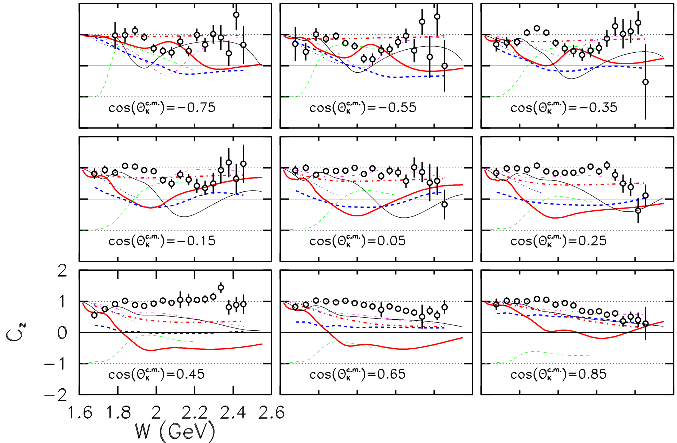
FIG. 6: (Color online) The observable C_z for the reaction \vec{\gamma} + p \rightarrow K^+ + \vec{\Lambda} , plotted as a function of the c.m. energy W . The circles are the results of this measurement, with uncertainties discussed in the text. The thin dashed (green) curves are from Kaon-MAID [10], the thick solid (red) curves are from SAP [18], the thick dashed (blue) curves are from BG [42], the thin solid (black) curves are from RPR [16], and the thick dot-dashed (magenta) curves are from GENT [12]. The thick dot-dashed (red) curves are from GLV [24, 25]. The thin dotted (blue) curves are from SLM [20].
