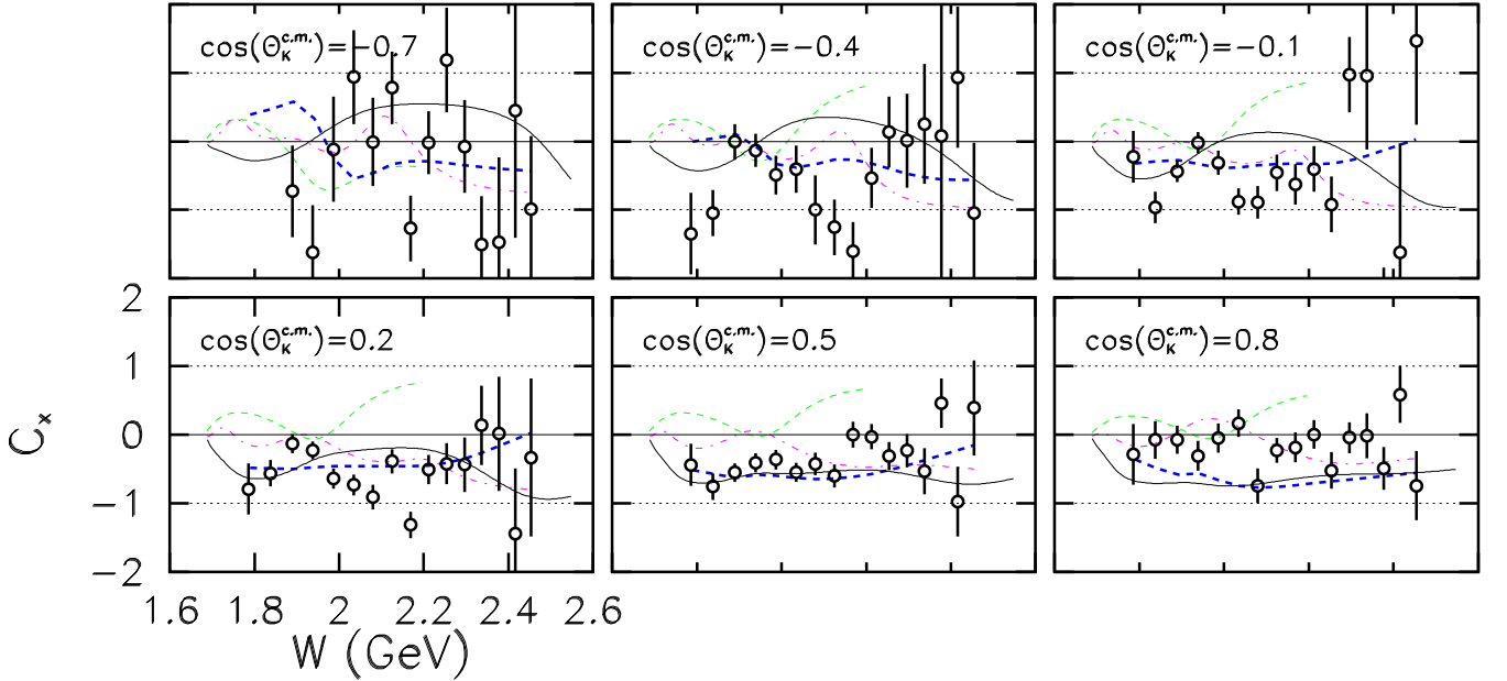
FIG. 14: (Color online) The observable C_x for the reaction \bar{\gamma} + p \rightarrow K^+ + \bar{\Sigma}^0 , plotted as a function of the c.m. energy W . The circles are the results of this measurement, with uncertainties discussed in the text. The thin dashed (green) curves are from Kaon-MAID [10], the thick dashed (blue) curves are from BG [42], the thin solid (black) curves are from RPR [16], and the thick dot-dashed (magenta) curves are from GENT [12].
