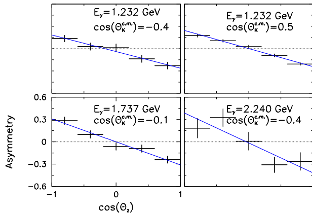
FIG. 3: (Color online) Representative hyperon yield asymmetries as a function of proton decay angle for the case of the C_z observable for the \Sigma^0 . The scales are the same in all plots.
