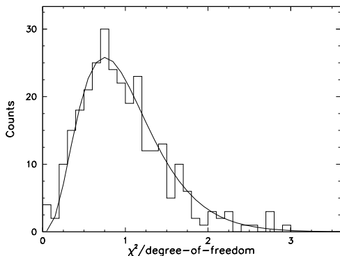
FIG. 4: (Color online) Distribution of the reduced \chi^2 values for fits with 8 degrees of freedom for the C_z fits in the K^+\Lambda case.
