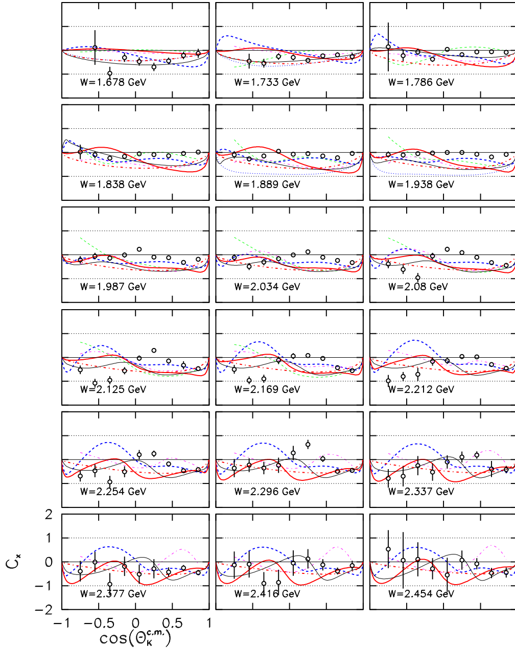
FIG. 9: (Color online) The observable C_x for the reaction \bar{\gamma} + p \rightarrow K^+ + \bar{\Lambda} , plotted as a function of the kaon angle. The 18 panels are for increasing values of W in steps of about 50 MeV. The circles are the results of this measurement, with uncertainties discussed in the text. The thin dashed (green) curves are from Kaon-MAID [10], the thick solid (red) curves are from SAP [18], the thick dashed (blue) curves are from BG [42], the thin solid (black) curves are from RPR [16], and the thick dot-dashed (magenta) curves are from GENT [12]. The thick dot-dashed (red) curves are from GLV [24, 25]. The thin dotted (blue) curves are from SLM [20].
