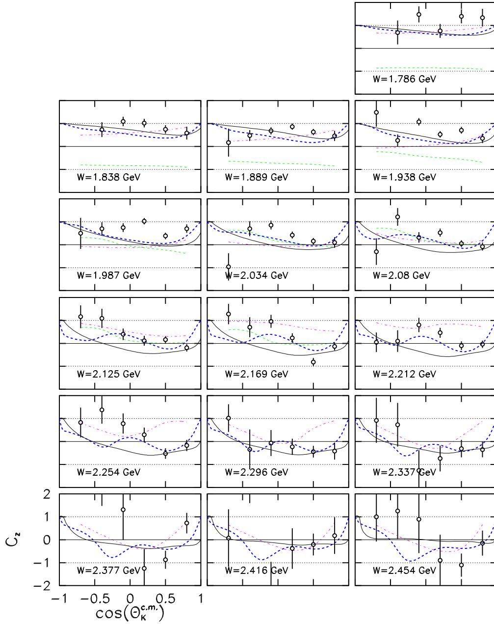
FIG. 15: (Color online) The observable C_z for the reaction \bar{\gamma} + p \rightarrow K^+ + \bar{\Sigma}^0 , plotted as a function of the kaon angle. The 16 panels are for increasing values of W in steps of about 50 MeV. The circles are the results of this measurement, with uncertainties discussed in the text. The thin dashed (green) curves are from Kaon-MAID [10], the thick dashed (blue) curves are from BG [42], the thin solid (black) curves are from RPR [16], and the thick dot-dashed (magenta) curves are from GENT [12].
