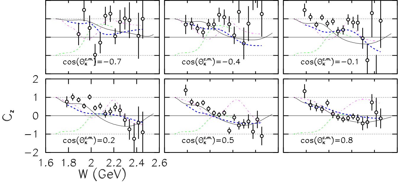
FIG. 13: (Color online) The observable C_z for the reaction \bar{\gamma} + p \rightarrow K^+ + \bar{\Sigma}^0 , plotted as a function of the c.m. energy W . The circles are the results of this measurement, with uncertainties discussed in the text. The thin dashed (green) curves are from Kaon-MAID [10], the thick dashed (blue) curves are from BG [42], the thin solid (black) curves are from RPR [16], and the thick dot-dashed (magenta) curves are from GENT [12].
