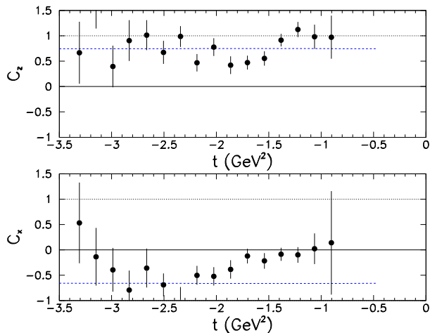
FIG. 12: (Color online) The observables C_z and C_x for the reaction \vec{\gamma} + p \rightarrow K^+ + \vec{\Lambda} , plotted as a function of t . The dashed (blue) curves are a prediction [31, 47] from perturbative QCD assuming helicity conservation at the quark level.
