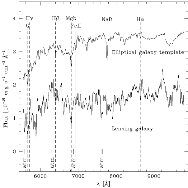
Fig. 2. Spectrum of the lensing galaxy. The total integration time is 5000 s. The template spectrum of a redshifted elliptical galaxy at z=0.317 is shown for comparison (Kinney et al. 1996). Atmospheric absorptions are indicated by the label atm.
