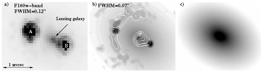
Fig. 3. Deconvolution of QJ 0158-4325 images (F160W). North is to the top, East to the left. a) Original image. b) Deconvolved image: the quasar images A and B appear as point sources, the lensing galaxy is the sum of a de Vaucouleurs profile plus the residuals which are not fitted by the light profile. The white contours trace the light distribution of the smooth objects (quasar host galaxy and flux residuals of the lensing galaxy). c) de Vaucouleurs luminosity profile of the lensing galaxy, with a lower flux cut than in image (b), in order to highlight its orientation and ellipticity.
