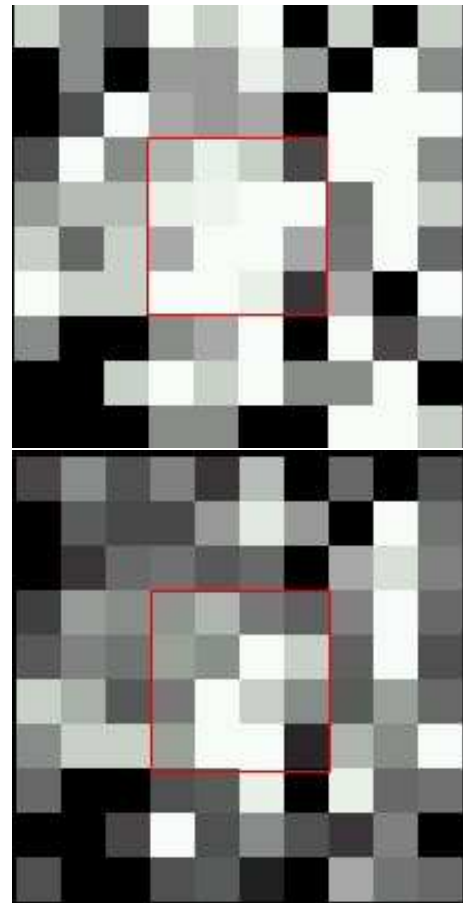
Fig. 4. The spectroscopic completeness for our high precision velocity sample in the inner 20' \times 20' . Top panel: galaxies brighter than R = 19.5 ; bottom panel: galaxies brighter than R = 20 . Individual cells are 2' \times 2' wide. The completeness ratio increases from black to white. The threshold value is 0.1 for black pixels and 0.6 for white pixels. The inner field ( 8' \times 8' ) is displayed as a red square.
