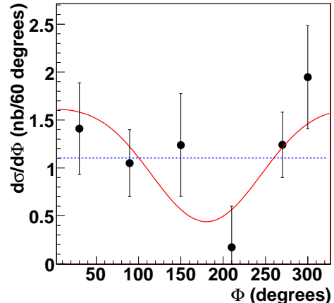
FIG. 12: (Color online) d\sigma/d\Phi vs \Phi . The curve shows a fit to Eq. 11 which is used to determine \sigma_{TT} and \sigma_{LT} . The dotted line is a fit to a constant function which is expected from SCHC.
