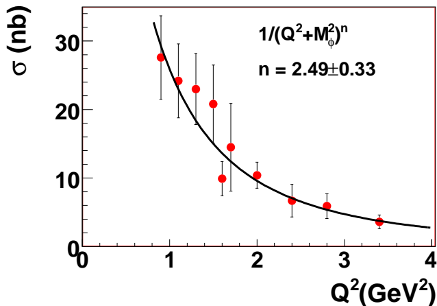
FIG. 16: (Color online) Fit to the cross section as a function of Q^2 distribution to determine scaling using data from the present experiment and CLAS data from Ref. [21].
