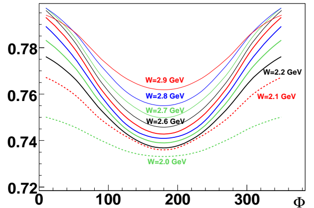
FIG. 10: (Color online) Plot of radiative correction F_{rad} as a function of \Phi for assorted values of W from 2.0 to 3.0 \text{GeV} . The correction for each W value was computed for \langle Q^2 \rangle = 2.47 \text{ GeV}^2 and \langle \cos\theta_{CM} \rangle = 0.345 .
