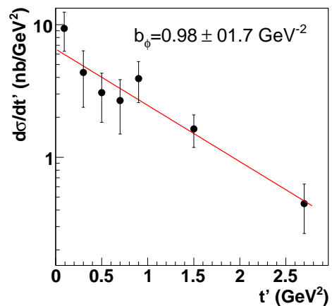
FIG. 11: (Color online) Plot of d\sigma/dt' along with an exponential fit.
