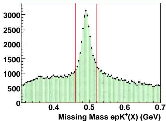
FIG. 4: (Color online) Distribution of epK^+X missing mass. The vertical lines indicate the cuts placed to select events with a missing K^- .
