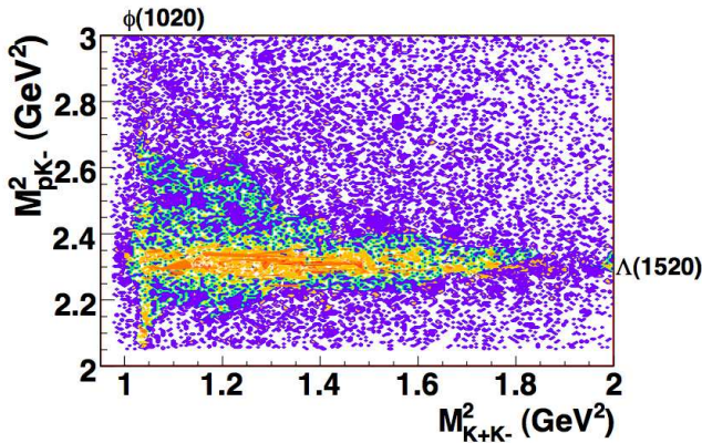
FIG. 7: Dalitz plot of M^2_{pK^-} versus M^2_{K^+K^-} . The well-defined orange/red horizontal strip is the \Lambda(1520) band. The vertical orange/red strip is the \phi(1020) band.
