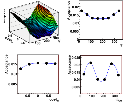
FIG. 9: (Color online) 2-D Acceptance in \cos\theta_H and \psi , as well as the 1-D acceptance in \cos\theta_H , \Phi , and \psi . Error bars are not shown; the lines are present to guide the eye.
