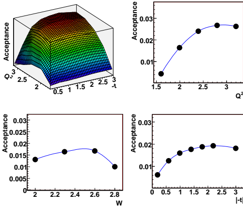
FIG. 8: (Color online) 2-D Acceptance in Q^2 and t , as well as the 1-D acceptance in Q^2 , W , and -t . Error bars are not shown; the lines are present to guide the eye.
