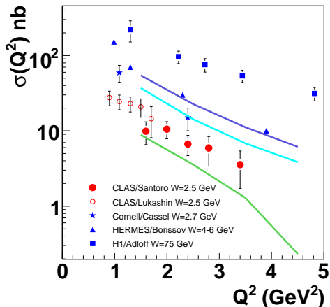
FIG. 15: (Color online) Total cross sections as a function of Q^2 for our data (red full circles), previous JLab data (open circles) [21], Cornell data (stars) for W between 2 and 3.7 GeV [20], HERMES data (triangles) for W between 4 and 6 GeV [22], and HERA data (squares) at high W [25]. The curves show the predictions of the JML model at W=2.9 , 2.45 and 2.1 GeV (top to bottom).
