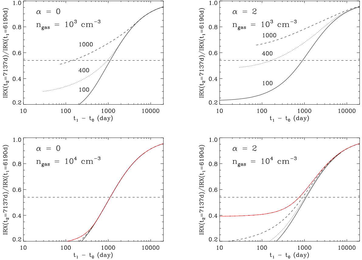
Fig. 9.— Evolution of the ratio IRX(t_2)/IRX(t_1) as a function of the time difference t_1 - t_0 . The time t_0 is the time since the explosion when the SN blast wave first encountered the dusty equatorial ring (ER), taken here to be the independent variable. The times t_1 and t_2 correspond, respectively, to days 6190 and 7137 since the explosion, the two epochs of near-simultaneous Spitzer and Chandra observations of the ER. The dashed horizontal line depicts the nominal value of the IRX(t_2)/IRX(t_1) ratio which is 0.53 \pm 0.16 (see Table 1). The curves are labeled by a_{max} , the maximum grain size (in Å) of the distribution. The minimum grain size was taken to be 10 Å in all cases. The red curves correspond to a narrow grain size distribution of the ER with \{a_{min}, a_{max}\} = \{0.023, 0.22\} \mu\text{m} . Figures are also labeled by the value of n_{gas} , the density of the shocked gas. Left column: A spherical blast wave expanding into a one-dimensional protrusion ( \alpha = 0 ). Right column: A spherical blast wave expanding into a uniform ISM ( \alpha = 2 ).
