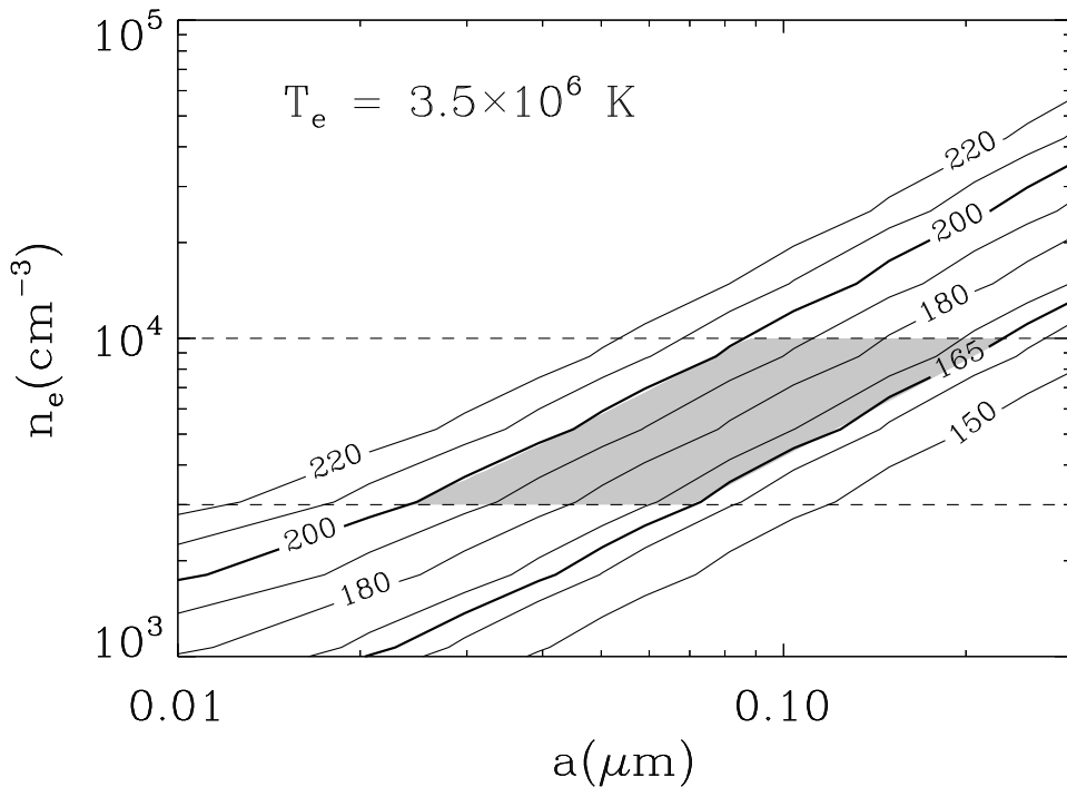
Fig. 8.— Contours of the dust temperature as function of gas density and grain size for the given electron temperature, T_e , of the soft X-ray component. For the range of electron densities constrained by the plasma ionization timescale (indicated by the dashed horizontal lines), the observed range of dust temperature (indicated by the thick contours) limits the grain size distribution to be between \sim 0.023 - 0.22 \mu\text{m} .
