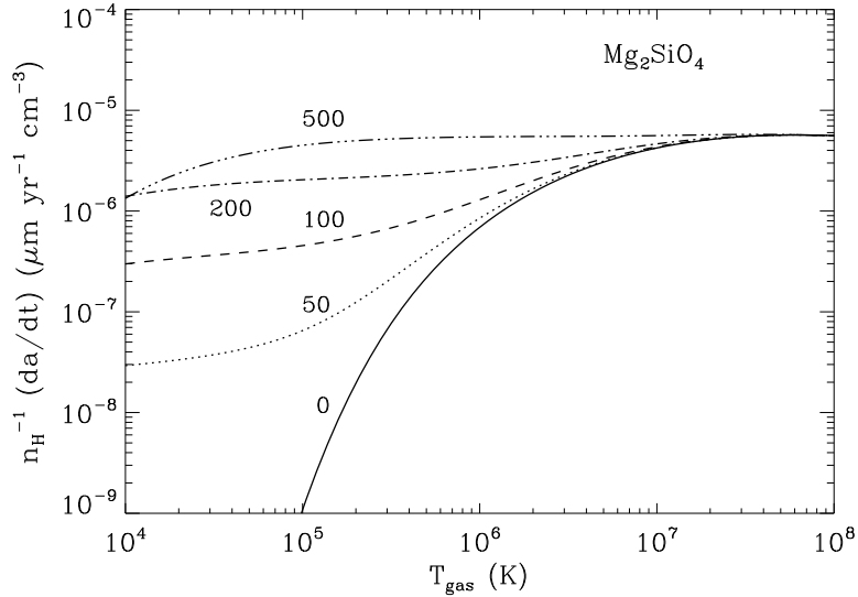
Fig. 4.— The absolute value of the sputtering rate (normalized to the H-number density) of silicate ( \text{Mg}_2\text{SiO}_4 ) dust grains moving through a hot gas of solar composition as a function of gas temperature. The curves are marked by the grain velocity (in \text{km s}^{-1} ).
