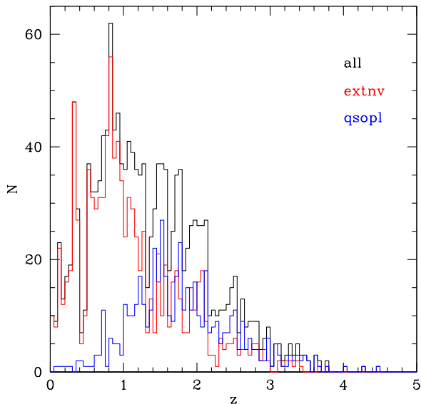
FIG. 6.— Photometric redshift distribution for the entire sample (black line), “extnv” (red) and “qsopl” (blue) samples.
