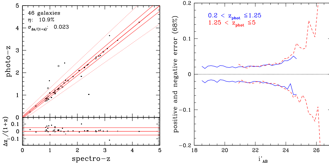
FIG. 12.— Left: Same as Figure 4 for the 46 sources with i_{AB}^+ > 22.5 with spectroscopic redshifts, which has been used for an a posteriori test. Right: 1- \sigma error for the z_{phot} estimate as a function of the apparent magnitude in the redshift range 0.2 < z_{phot} \leq 1.25 (blue) and 1.25 < z_{phot} \leq 5 (red).
