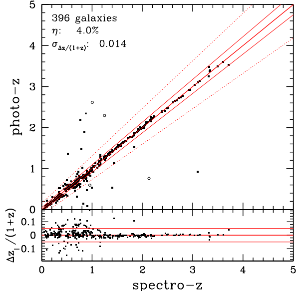
FIG. 4.— Comparison of photometric and spectroscopic redshifts for the 396 sources with i_{AB}^* < 22.5 . Empty circles represent sources for which the second peak in the redshift probability distribution agrees with the spectroscopic redshift. The lines correspond to 1) z_{phot} = z_{spec} (thick solid), 2) z_{phot} = z_{spec} \pm 0.05(1+z_{spec}) (solid) and 3) z_{phot} = z_{spec} \pm 0.15(1+z_{spec}) (dotted).
