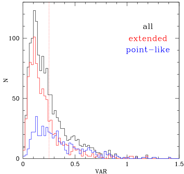
FIG. 2.— Histogram of the parameter VAR for all the sources (black solid line) extended (red) and point-like sources (blue). The vertical dotted line at VAR =0.25 defines our adopted separation between host (low VAR ) and AGN (high VAR ) dominated sources.
