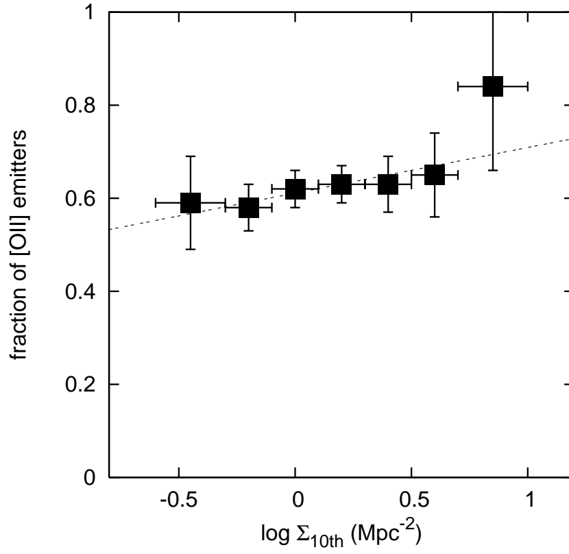
FIG. 3.— The fraction of [O II] emitters is plotted as a function of the galaxy local density. The dotted line shows the linear fit to the data. The star-formation activity is more active in higher density regions. Here the adopted size of the \log \Sigma_{10\text{th}} bin is 0.2 dex, except for the lowest- and highest- \log \Sigma_{10\text{th}} bins where there are only a few objects (0.3 dex for these bins).
