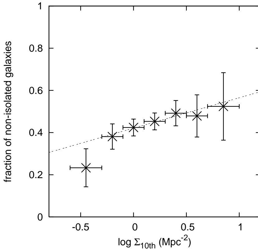
FIG. 5.— The fraction of non-isolated galaxies among [O II] emitters is plotted as a function of the galaxy local density. The dotted line shows the linear fit to the data. Here the adopted size of the \log \Sigma_{10\text{th}} bin is 0.2 dex, except for the lowest- and highest- \log \Sigma_{10\text{th}} bins where there are only a few objects (0.3 dex for these bins).
