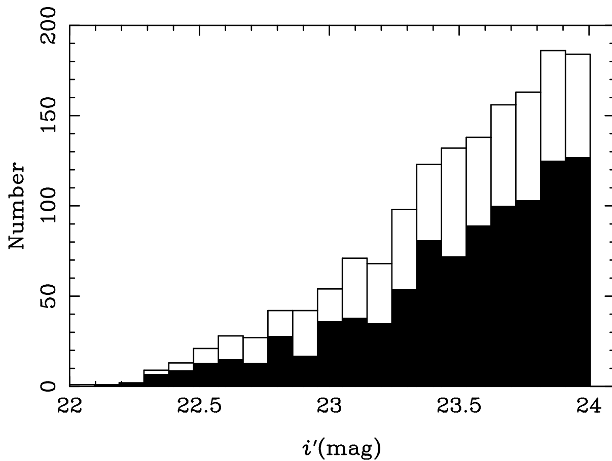
FIG. 2.— The number count of our sample as a function of i' magnitude. Open boxes denote our total sample, including both [\text{O II}] emitters and non emitters. Filled boxes denote [\text{O II}] emitters.
