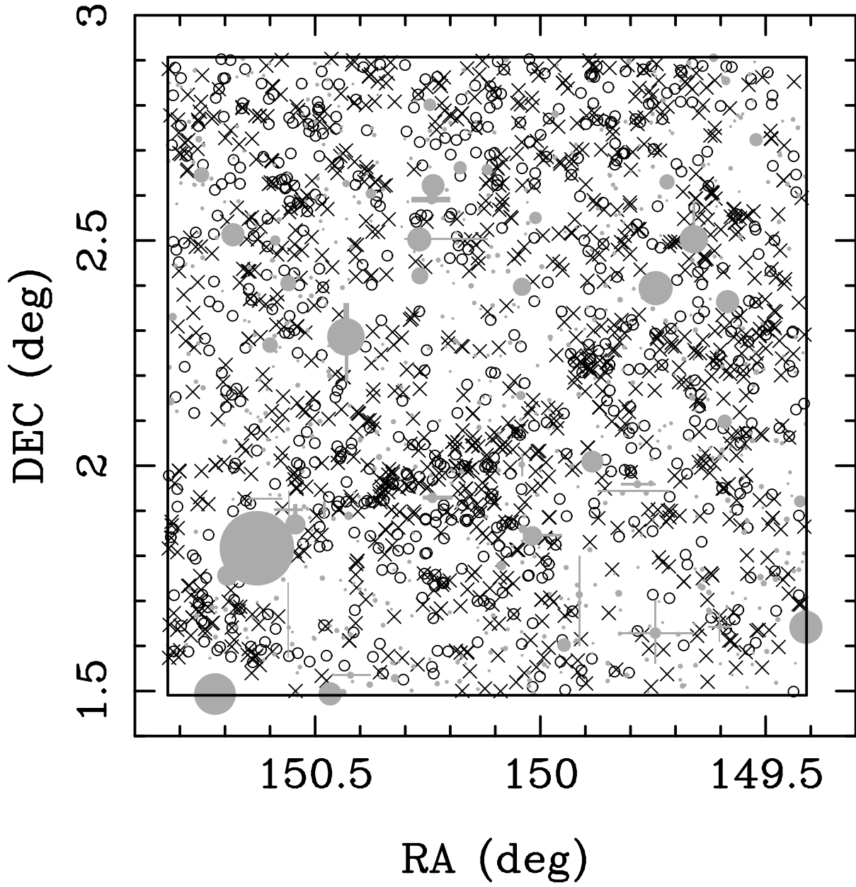
FIG. 1.— Spatial distributions of our sample at 1.17 < z < 1.20 in the COSMOS field. Open circles denote non-emitters in our sample. Cross symbols denote [O II] emitters selected by Takahashi et al. (2007) in our sample. The circle areas are masked out for the detection. We select galaxies in the region of the large solid square: 149^{\circ}.40917 < \text{RA (J2000)} < 150^{\circ}.82680 and 1^{\circ}.49056 < \text{Dec (J2000)} < 2^{\circ}.90705 (Takahashi et al. 2007).
