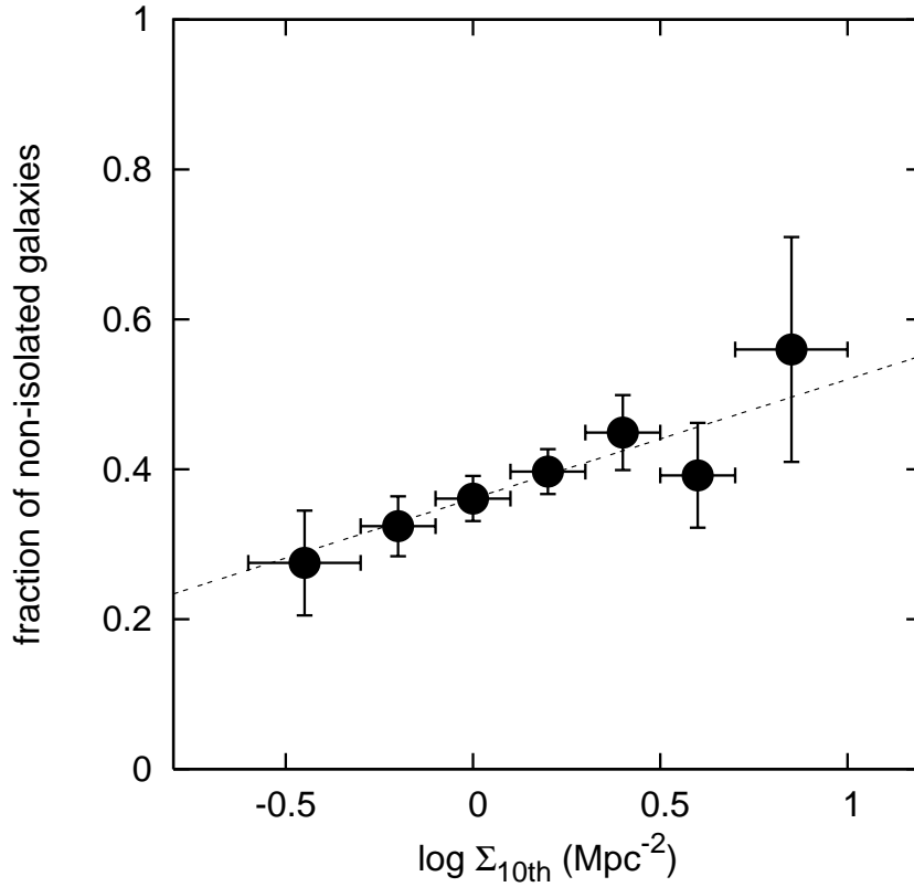
FIG. 4.— The fraction of non-isolated galaxies is plotted as a function of the galaxy local density. The dotted line shows the linear fit to the data. Here the adopted size of the \log \Sigma_{10\text{th}} bin is 0.2 dex, except for the lowest- and highest- \log \Sigma_{10\text{th}} bins where there are only a few objects (0.3 dex for these bins).
