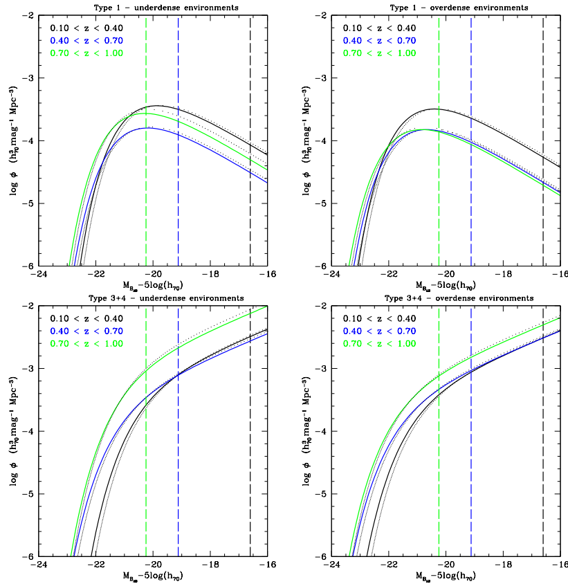
Fig. 9. Evolution of the luminosity functions for different galaxy types in different environments (low density on the left, high density on the right): type 1 (upper panels) and type 3 + 4 (lower panels) galaxy samples. The color refer to different redshift ranges: [0.10 - 0.40] in black, [0.40 - 0.70] in blue and [0.70 - 1.00] in green. The STY estimates are derived with \alpha fixed. The meaning of lines is the same as in Fig. 3: points from the C^+ estimates are not reported for clarity.
