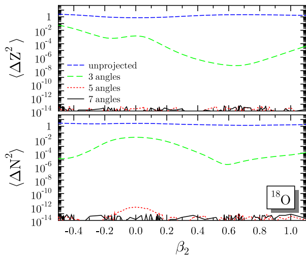
FIG. 3: (Color online) Dispersion of the proton and neutron number of the unprojected SR state and the particle-number projected SR using 3, 5 or 7 discretization points of the gauge-space integrals as a function of their deformation. For 5 points the projected state is sufficiently converged, for 7 and more points (not shown) the dispersion cannot be distinguished from numerical noise.
