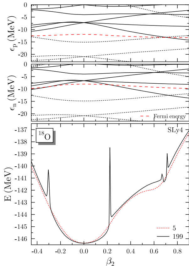
FIG. 1: (Color online) Particle-number restored deformation energy surface of ^{18}\text{O} calculated with SLy4 and a density-dependent pairing interaction and the corresponding single-particle spectra of protons and neutrons as a function of the axial quadrupole deformation for L = 5 and 199 discretization points of the integral over the gauge angle (lowest panel). There are clear anomalies that appear when either a proton or neutron single-particle level crosses the Fermi energy. The dimensionless quadrupole deformation \beta_2 is defined in Eq. (66).
