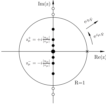
FIG. 2: Schematic view of the analytical structure of the transition densities defined in Eqs. (38-40) and of the PNR functional energy kernel \mathcal{E}[\varphi] in the complex plane. Poles marked with filled circles are within the standard circular integration contour of radius R = 1 , while those outside are marked with open circles. The cross marks the location of the SR energy functional at z = 1 . The operator e^{i\varphi N} produces a rotation in gauge space, while e^{\eta N} is a shift transformation as defined in Eq. (45).
