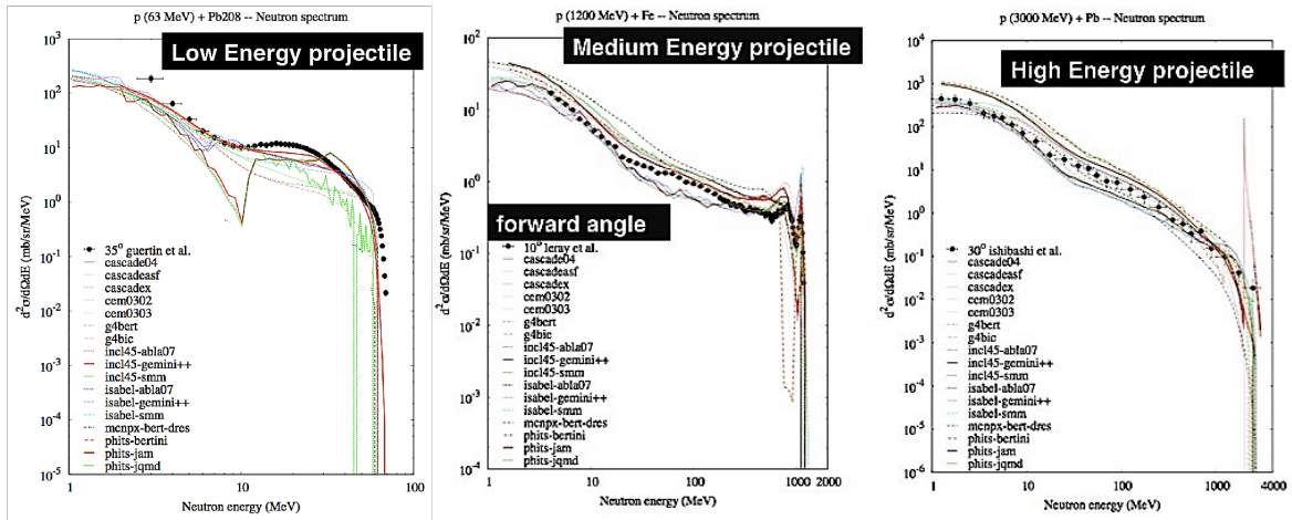
Fig. 2. Neutron spectra at particular angles for three reactions. From left to right: p(63 MeV)+Pb (35°), p(1.2 GeV)+Fe (10°) and p(3 GeV)+Pb (30°). All models are plotted.
