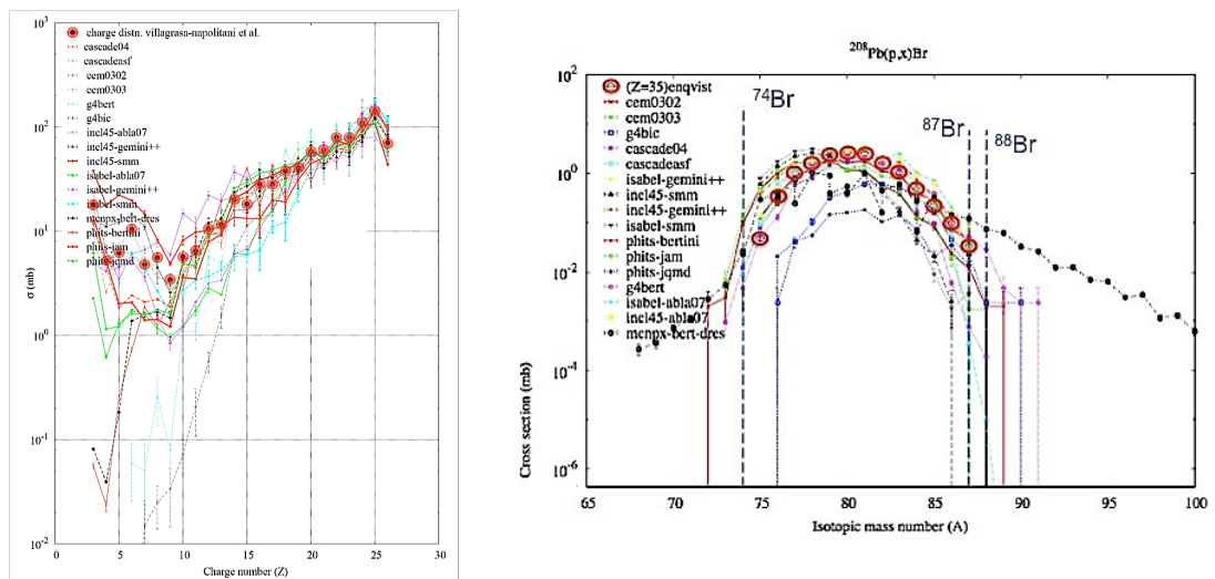
Fig. 6. Charge distribution ( ^{56}\text{Fe}(1 \text{ GeV} \cdot \text{A})+^1\text{H} ) on the left part and on the right part Br mass distribution from ^{208}\text{Pb}(1 \text{ GeV} \cdot \text{A})+^1\text{H} . All models are plotted.
