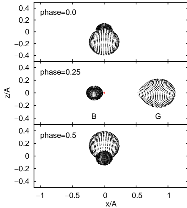
Figure 10. Representation of the B and G-star of AU Mon pictured in three different phases. The cross in the middle panel denotes the center of mass. The system does not show a total eclipse.
