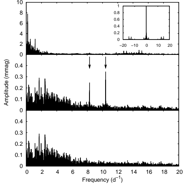
Figure 13. The periodogram of the residuals out of primary eclipse together with the spectral window (top+inset). The middle panel shows the periodogram after prewhitening for 9 low-frequency signals. The bottom panel shows the final residual periodogram after prewhitening all significant frequency peaks.
