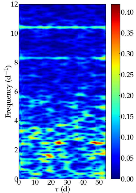
Figure 14. The Short Time Fourier Transform of the residuals of the CoRoT light curve after prewhitening for the orbital frequency. The units of the colour scale are in mmag. See text for details.
