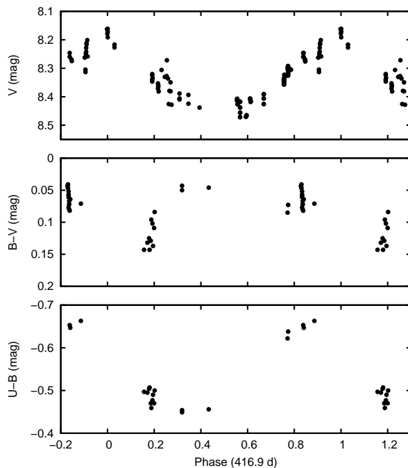
Figure 3. The V magnitude of AU Mon outside minima plotted vs. phase of the 417-d period (top). The B – V and U – B colour changes along the 417-d cycle of AU Mon are shown in the middle and bottom panel (see Sect. 8 for details).
