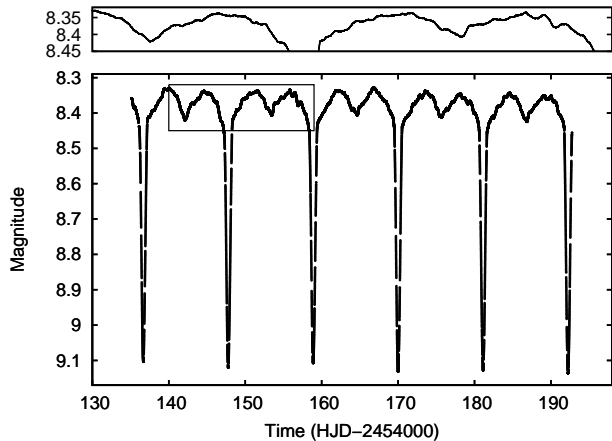
Figure 1. The complete CoRoT light curve of AU Mon. The upper panel shows an enlarged segment of the curve with very clear rapid non-orbital variations. The noise on the data is smaller than the symbol.
