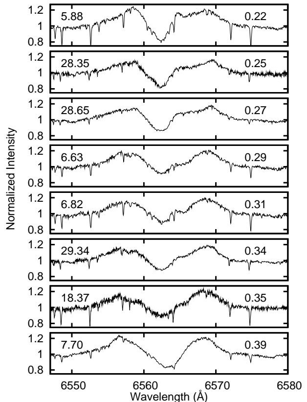
Figure 12. A sequence of the H\alpha line profiles showing a complicated velocity field and cycle-to-cycle variations. Data from 3 consecutive orbital cycles can be seen. In the left corner of each plot we list the time of measurement (HJD-2454100), in the right corner we give the orbital phase calculated from ephemeris (2).
