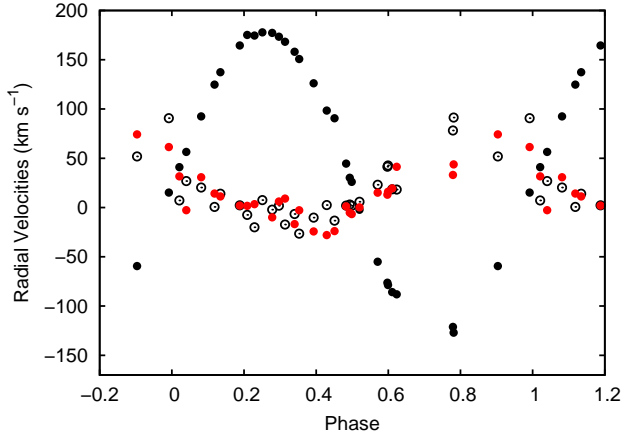
Figure 4. The RV curves of the late-type G-spectrum (black dots), B-spectrum (open circles) and the H\alpha emission wings (red dots) measured in SPEFO. One can see that the B-spectrum RV, based on the He I 5876 Å, and that of the H\alpha emission wings, define similar RV curves which are both shifted in phase with respect to the expected RV curve of the G-component.
