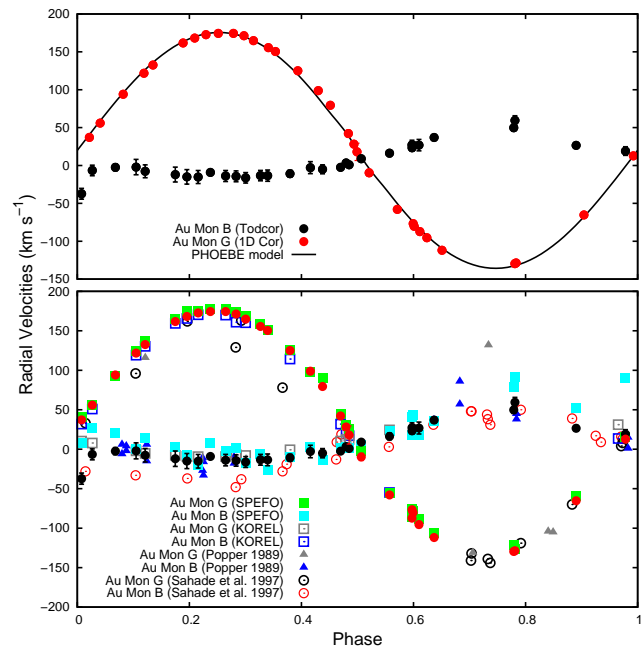
Figure 7. Radial velocities obtained in this study by various methods (SPEFO, TODCOR, 1D CC, KOREL) compared to published values. The top panel shows our new and final RVs for sake of clarity, the bottom panel shows the comparison. The black line shows the final PHOEBE model for the G-star. The residuals for the G-star are pictured in Fig. 11.
