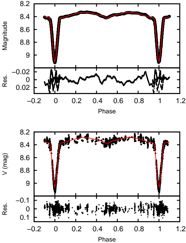
Figure 8. The final PHOEBE model plotted in red on top of one part of the CoRoT light curve (top) and the V-band light curve (bottom), after removal of the long-term period of P_{\text{long}} = 417 \pm 8 days, phased against the period of 11.1130374 days. Below each light curve the residuals of the model and observations are shown.
