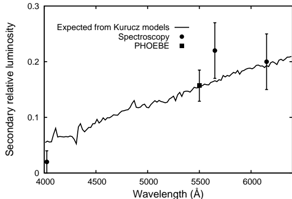
Figure 6. The expected wavelength dependence of the relative luminosity of the G-star to the total light of the system. We assumed effective temperatures of 15000 K and 5750 K for the B primary and the G secondary, respectively. The full line is based on Kurucz’ models. The light contribution at 6150 Å was fixed at 0.2. The luminosity ratio was estimated from detailed comparisons of the observed and synthetic spectra at several distinct wavelength regions and these values are shown by black dots with errors. The black square with an error box represents the luminosity ratio in the V band based on the PHOEBE solution.
