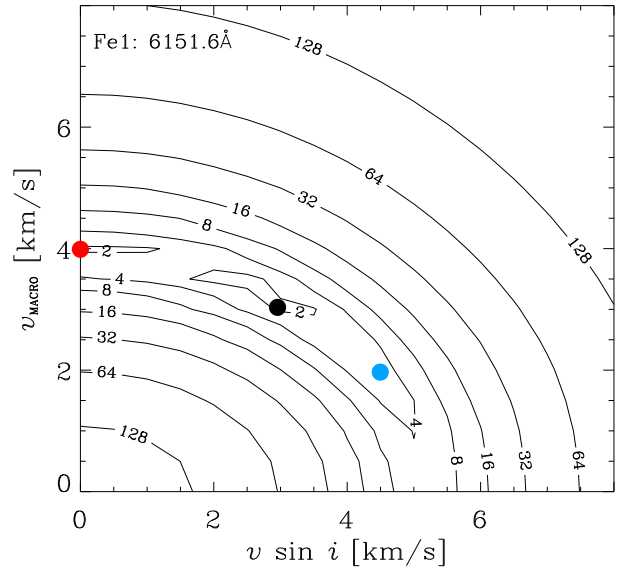
Fig. 2. Example of the \chi^2 contour surface used to determine v \sin i and v_{\text{macro}} for the Fe I line \lambda 6151.6 \text{ Å} . The three circles mark the minimum of the surface and the 1\text{-}\sigma uncertainty range. The corresponding three synthetic spectra are compared to the observed line in Fig. 3.
