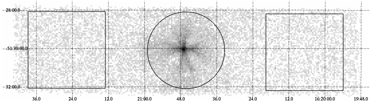
Fig. 1.— Image of IGR J16207–5129 as captured with the XIS1 detector on Suzaku . Pixels have been grouped in blocks of 4 (bin: group4 in ds9). The circular source and squared background selection regions are also shown.
