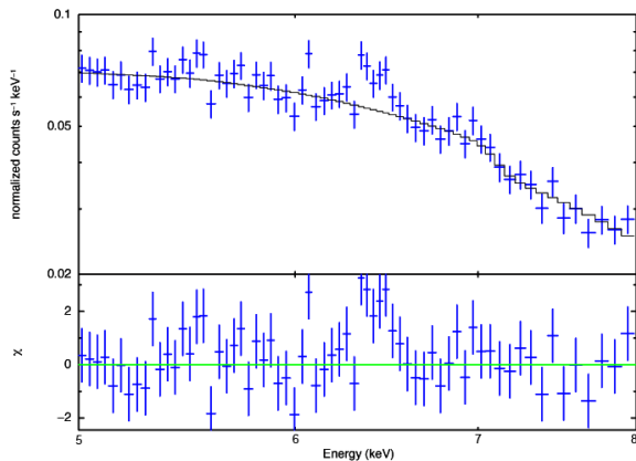
Fig. 5.— Combined XIS0 and XIS3 spectrum of IGR J16207–5129 in the 5–8 keV energy range. Each bin collects 150 counts. An absorbed power law was fit to the data (solid curve). An iron line at 6.4 keV is suggested by the residuals to the model displayed in the bottom panel.
