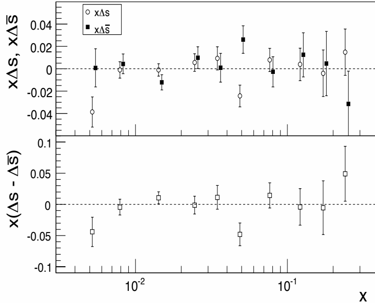
Figure 6.2: Results for the strange and anti-strange quark helicity distributions \Delta s and \Delta \bar{s} and the corresponding values of the difference \Delta s - \Delta \bar{s} as a function of the Bjorken variable x . Values are obtained from experimental asymmetries measured at \langle Q^2 \rangle = 3 and using the MRST parametrization for PDFs and the DSS parametrization for the fragmentation functions.
