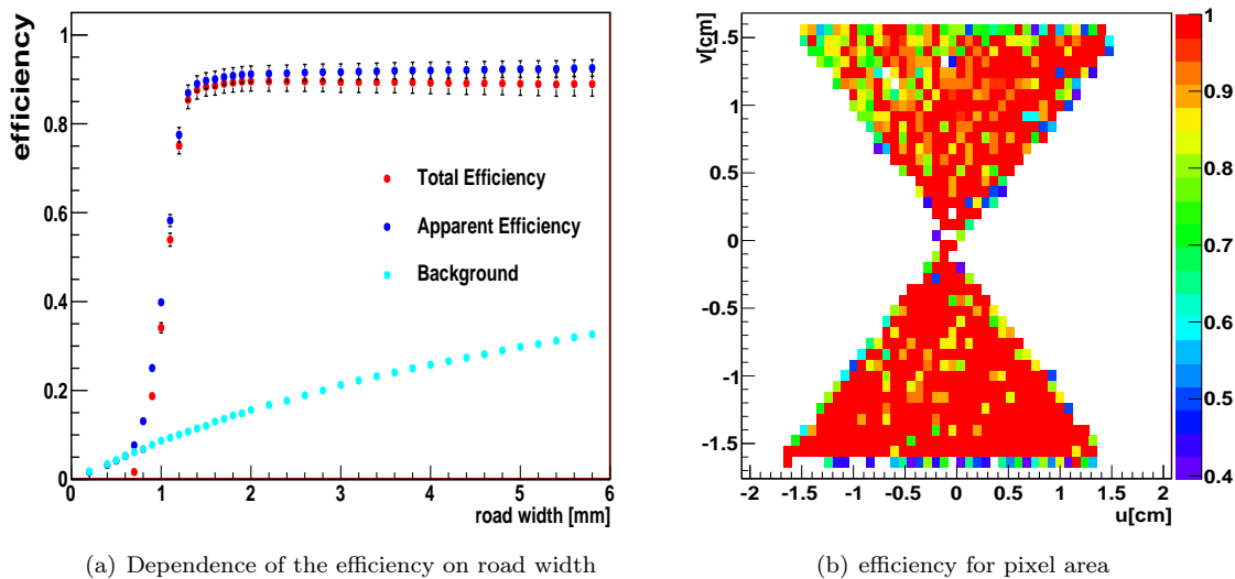
Figure 5.19: (a) Road width dependence of the efficiency for the strips for the voltage settings 410 V in low beam intensity for the bulk prototype. (b) 2-dimension efficiency for the pixel area of the bulk prototype.
