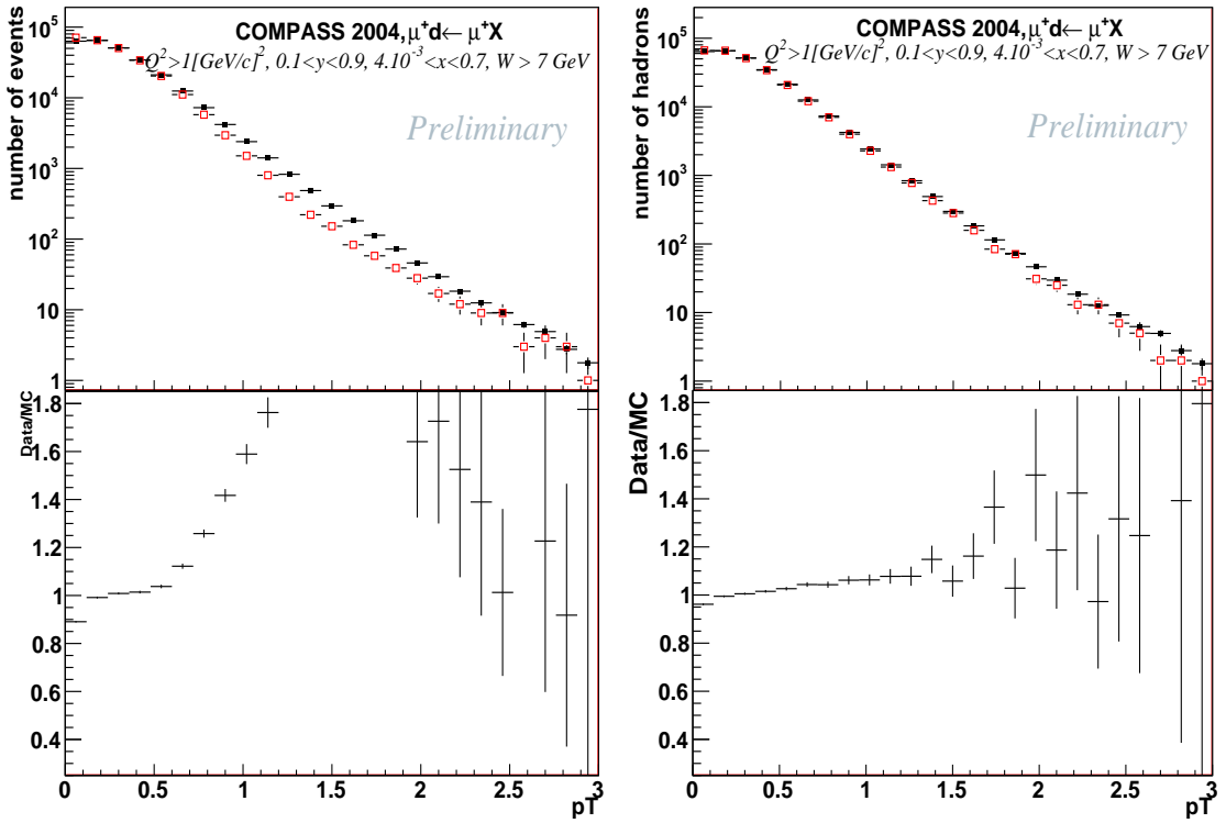
Figure 7.13: Upper row: Comparison of raw data (black) (corrected for radiative effects) and reconstructed MC data (red) for the transverse momentum P_T in the interval [0, 3] for the default (left) and the high P_T (right) tuning. Lower row: Ratio Data/MC.
