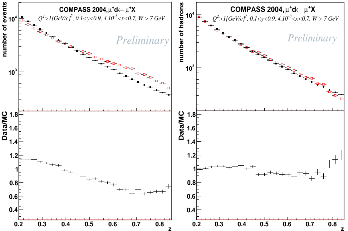
Figure 7.14: Upper row: Comparison of raw data (black, corrected for radiative effects) and reconstructed MC data (red) for the z variable in the range [0.2, 0.85] for the default (left) and the high P_T (right) tuning. Lower row: Ratio Data/MC.
