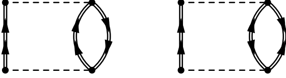
FIG. 2: Second-order normal self-energies \Sigma^{11(2')} (left) and \Sigma^{11(2'')} (right). See Fig. 1 for conventions.
