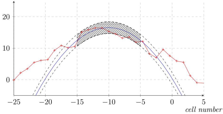
Figure 6.13 – Parabolic fit (—) of a noisy Gaussian pulse (—+). The noise amplitude on the cross-correlation plot defines a region (in gray) and thus there is an uncertainty on the extremum location.
