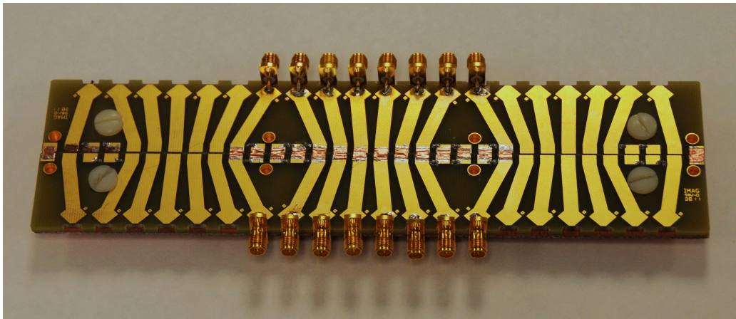
Figure 5.26 – Photograph of two fan-out boards attached together (for calibration measurements). Near the SMA connectors, the metal geometry inspired from the previous copper work (Figure 5.25) is visible.
