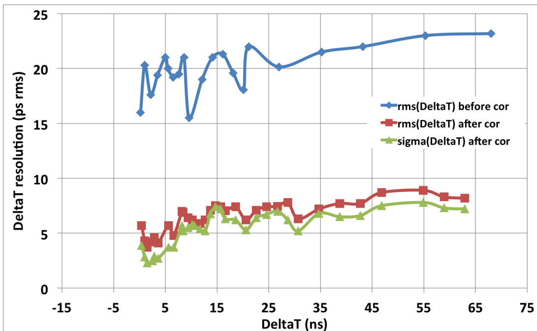
Figure 9.17 – Measurement of the time delay estimation between two pulses delayed from 0 to 65ns. We report here a sub-10ps RMS precision across the entire range.
