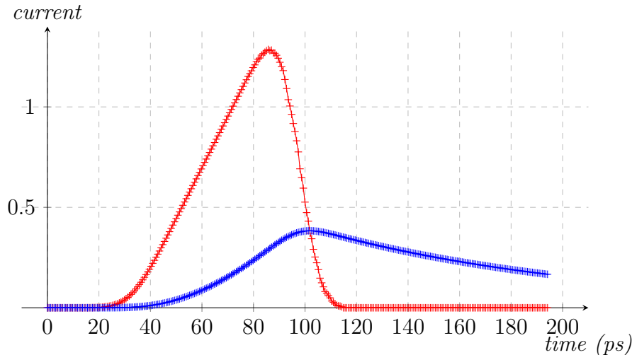
Figure 5.28 – Simulation of the pulse degradation due to the anode frequency limitation. The current excitation of the anode is plotted in red ( -\!-\!+ ) and the response of the anode is plotted in blue ( -+ ) for a cutoff frequency of 2 GHz.
