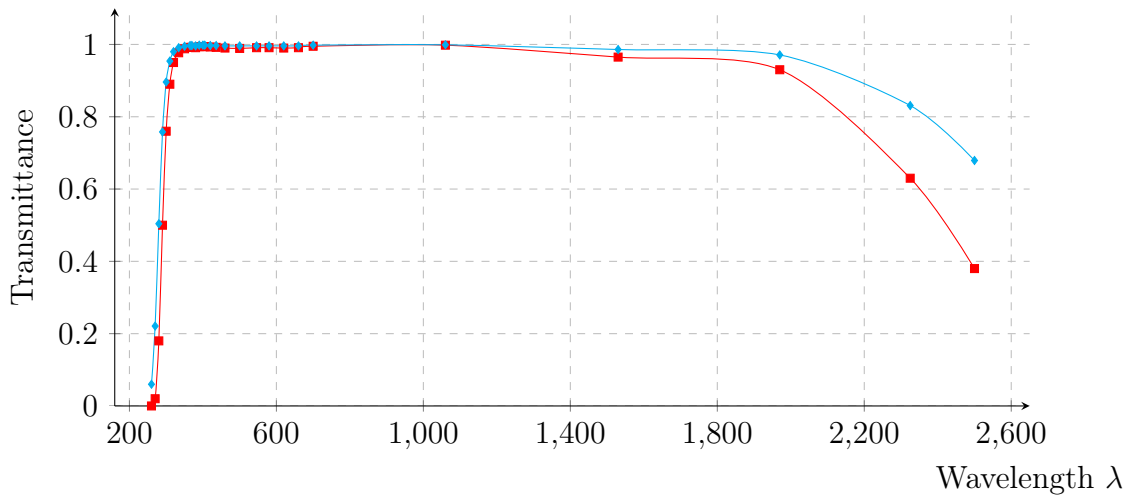
Figure 5.5 – Transmission of the NF-K5 glass from Schott [11] for a thickness of 10mm ( \color{blue}\blacktriangleleft ) and 25mm ( \color{red}\blacksquare ).
