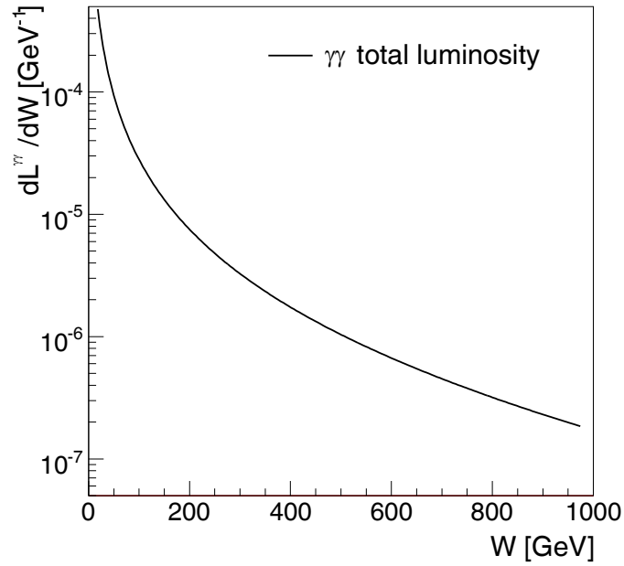
Figure 4.3 – Relative effective luminosity \gamma\gamma in pp collision versus the invariant mass of the two photons. The maximum virtuality of the two photons is set at Q_{max}^2 = 2GeV^2 [6].
