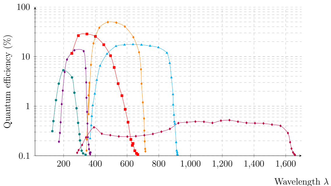
Figure 5.10 – Quantum efficiency versus wavelength of various photocathodes: Cs-Te ( \bullet ), GaN ( \blacklozenge ), SuperBialkali ( \blacksquare ), GaAsP ( \blacktriangle ), GaAs ( \blacklozenge ), InP ( \blacklozenge ). Quantum efficiency is the ratio of photoelectrons emitted from the photocathode to the number of incident photons, expressed in percent.
