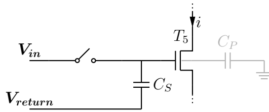
Figure 8.86 – Schematic of the equivalent circuit if the sampling cell was connected directly to the ADC comparator.
