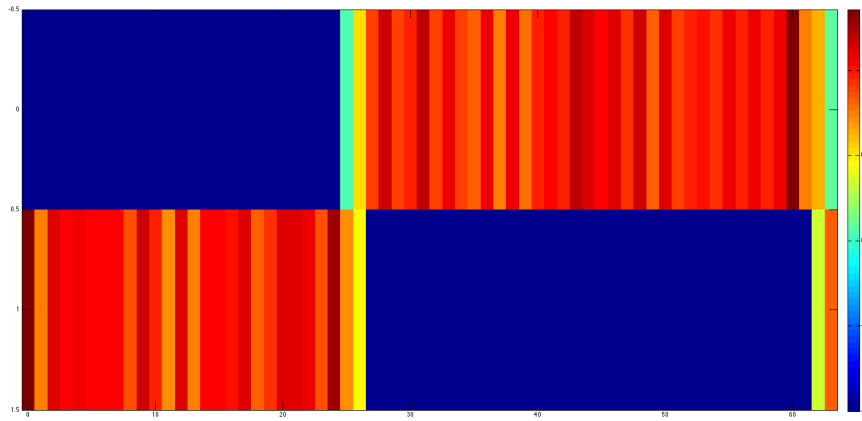
Figure 9.9 – Hit map of TB - TA along the 64 cells in SamPic, the sampling is done from left to right. In the first part (cells 1 to 25) TA = TB + 1 , then TA = TB (from cells 28 to 62) the metastability zones are cells 27, 28 and cells 63, 64.
