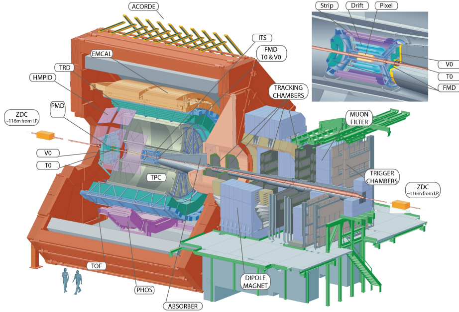
Figure 2.2: Schematic of the ALICE detector.
