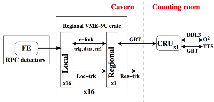
Figure 4.8: Schematic of the MID readout electronics architecture [226].
