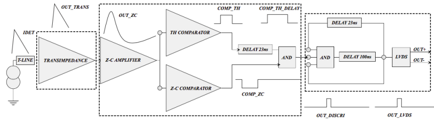
Figure 4.9: Block diagram of the FEERIC[227].
