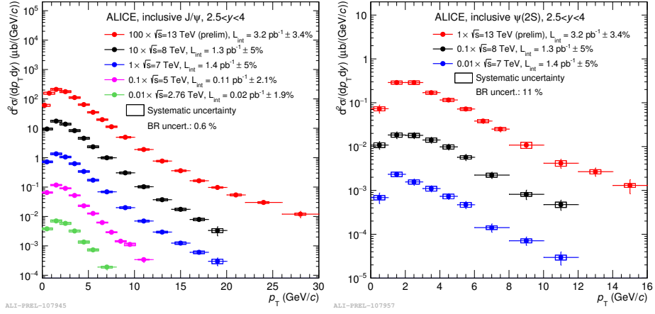
Figure 1.19: J/\psi production cross-section in pp collisions at \sqrt{s}=2.76, 5, 7, 8, and 13 TeV (left) and \psi(2S) production cross-section in pp collisions at \sqrt{s}=7, 8, and 13 TeV (right) as a function of p_T [147].
