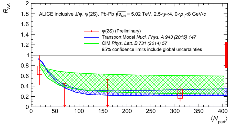
Figure B.1: Nuclear modification factor R_{AA} versus N_{\text{part}} compared to the Transport Model (in blue) and the Comover Interaction Model (in green). For the centrality bins where the signal could not be extracted, only the 95% confidence limit is shown. The global systematic uncertainty is drawn in the box around unity. The global uncertainties are already included in the confidence limit calculation.
