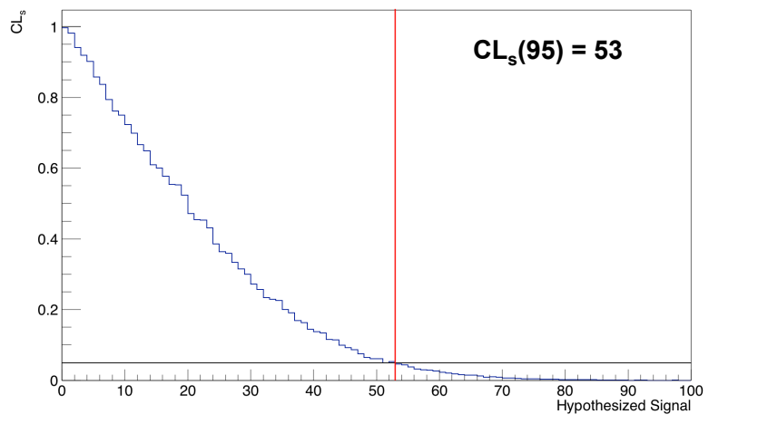
Figure 3.18: Example search for the signal value such as CL_s \leq 0.05 . In this example, b = 500 , the actual number of observed events is n_{data} = 510 and values of s are tested from 0 to 100. The upper limit is found when CL_s = 0.05 . It can be noted that by construction, CL_s = 1 for a hypothesis s = 0 , since it corresponds to the background only hypothesis.
