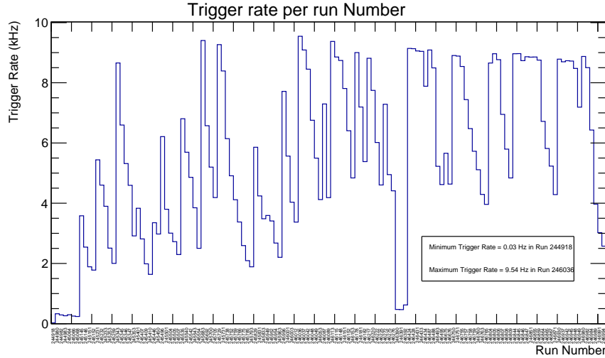
Figure 4.10: Minimum Bias trigger rate in Pb – Pb collisions at \sqrt{s_{\text{NN}}} = 5.02 TeV as a function of the run number.
