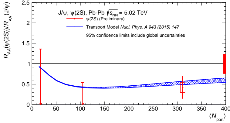
Figure 3.28: Double Ratio R_{AA}^{\psi(2S)}/R_{AA}^{J/\psi} as a function of N_{\text{part}} compared to the Transport Model. For the centrality bins where the signal could not be extracted, only the 95% confidence limit is shown. The global systematic uncertainty is drawn in the box around unity. The global uncertainties are already included in the confidence limit calculation. Uncertainties in the model correspond to different importances in the shadowing: the upper limit corresponds to 0% of shadowing and the lower limit corresponds to a shadowing of up to 20% for the most central collisions.
