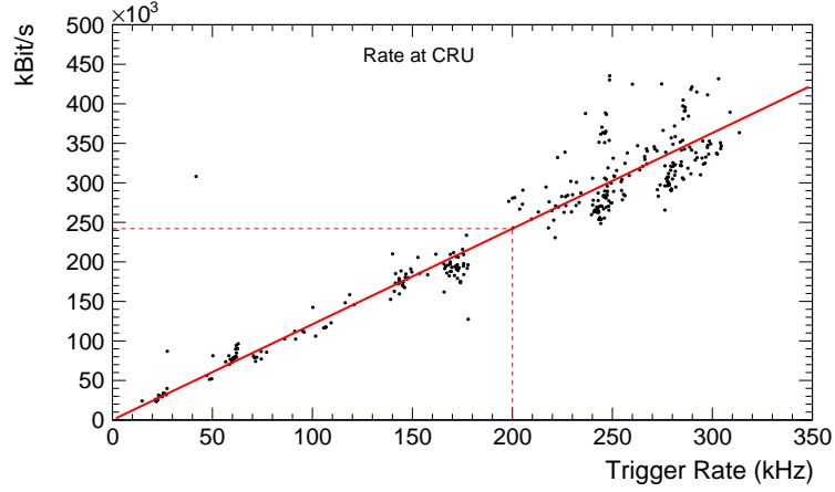
Figure 4.16: Data Flow to the CRU as a function of the trigger rate for all the pp runs. The values are fitted with a linear function to evaluate the value at 200kHz.
