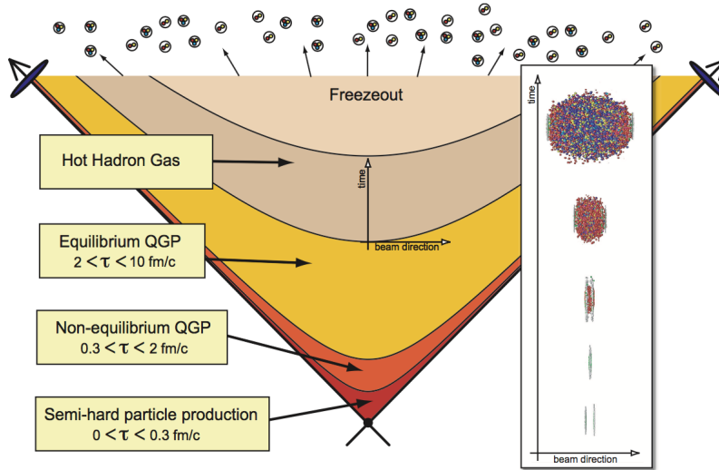
Figure 1.6: Illustration of the space-time evolution of the QGP as generated in a heavy ion collision at LHC energies. The overlay on the right shows the lab-frame evolution [60].
