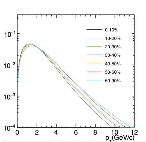
Figure 3.10: Simulated acceptance \times efficiency corrected J/\psi p_T distributions in seven centrality bins.
