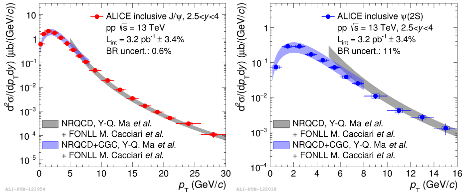
Figure 1.20: J/\psi (left) and \psi(2S) (right) production cross-sections in pp collisions at \sqrt{s} = 13 TeV compared to NLO NRQCD summed with FONLL calculations (grey) and LO NRQCD summed with FONLL calculation and CGC (blue) [147].
