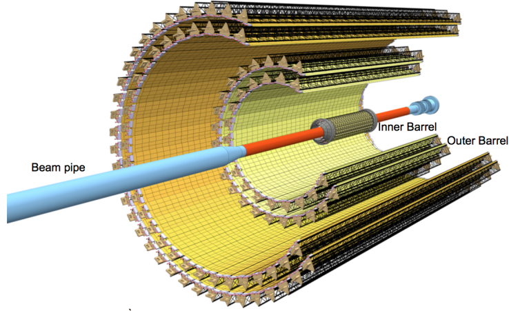
Figure 4.4: Layout of the new ITS detector [227].
