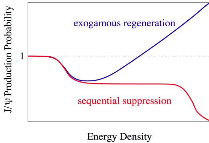
Figure 1.15: Illustration of the regeneration phenomenon [81].
