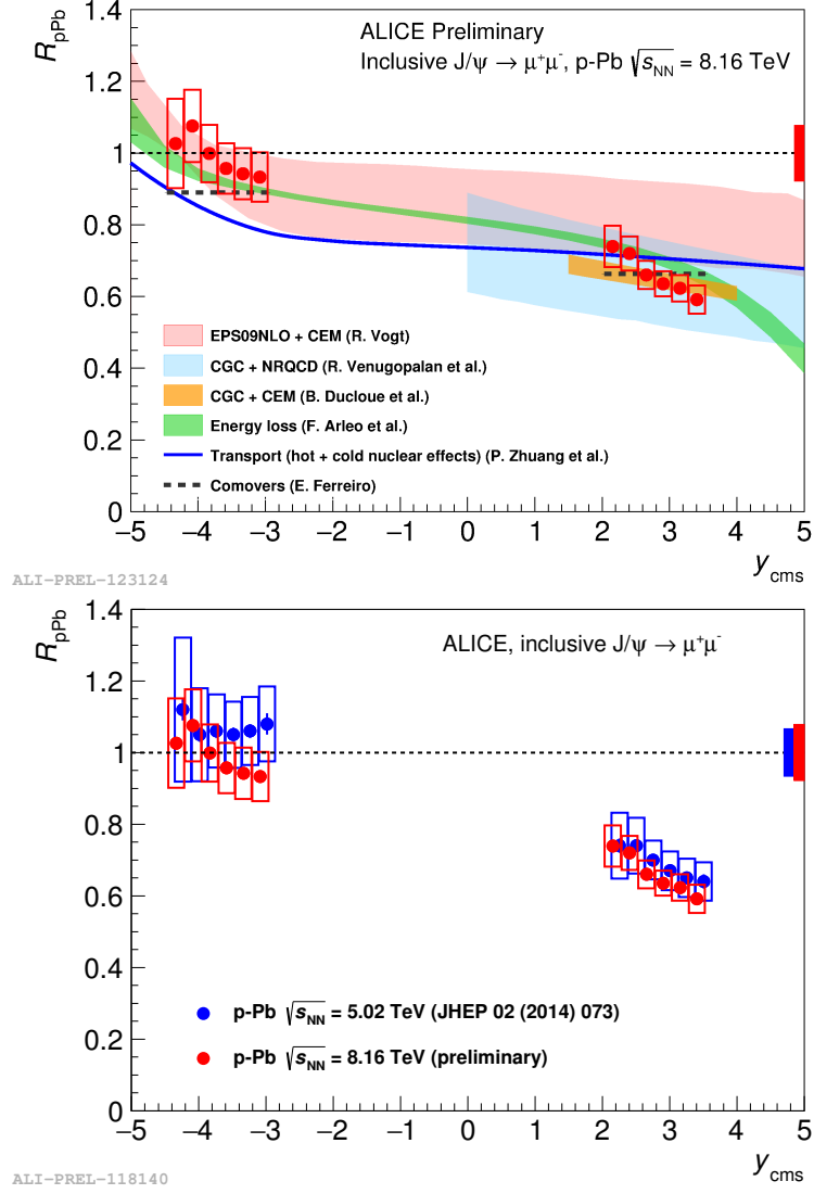
Figure 1.23: J/\psi R_{pA} at \sqrt{s_{\text{NN}}} = 8.16 TeV as a function of y compared to models (top) and with results at \sqrt{s_{\text{NN}}} = 5.02 TeV (bottom) [155].
