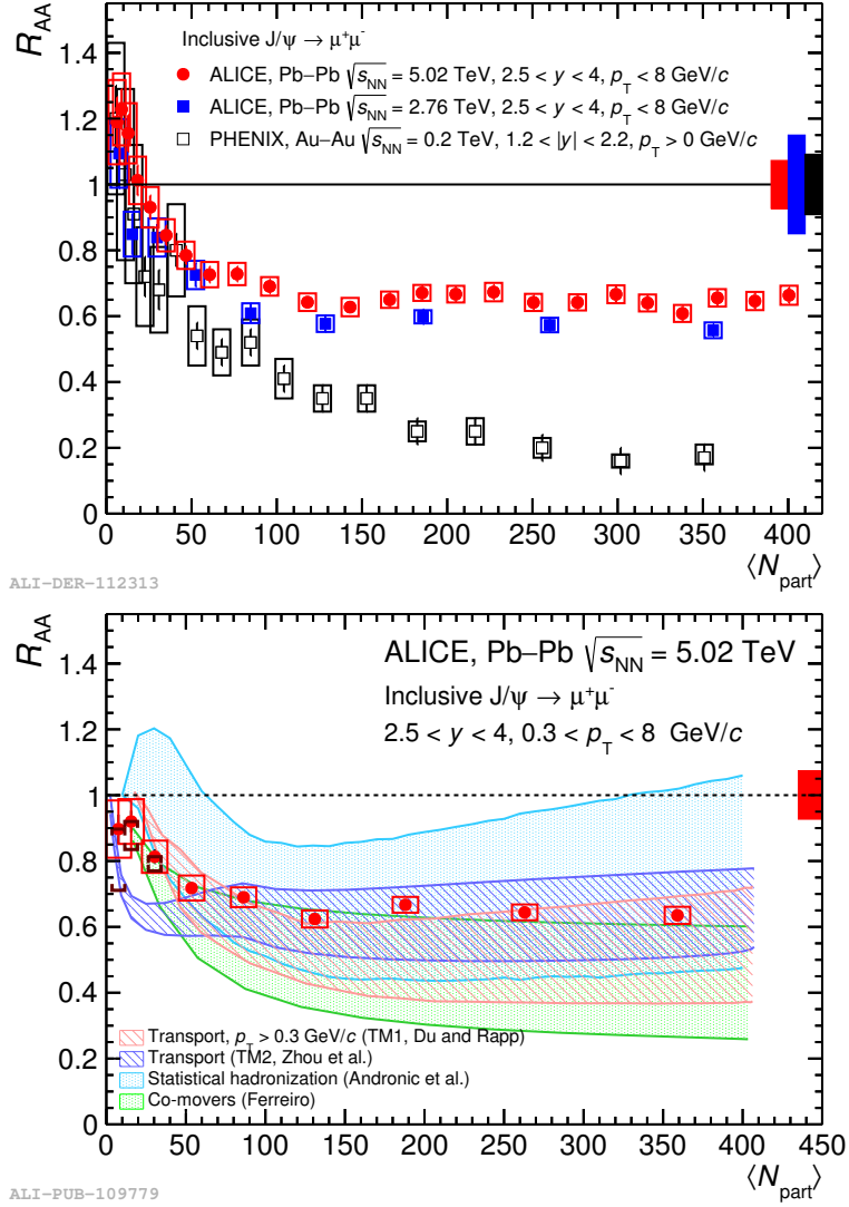
Figure 1.25: Top: Inclusive J/\psi R_{AA} as a function of N_{part} measured in Pb-Pb collisions at \sqrt{s_{NN}} = 2.76 TeV and \sqrt{s_{NN}} = 5.02 TeV compared to PHENIX measurement in Au-Au collisions at \sqrt{s_{NN}} = 0.2 TeV [156, 157]. Bottom: Inclusive J/\psi R_{AA} as a function of N_{part} with a cut p_T > 0.3 GeV/c measured in Pb-Pb collisions at \sqrt{s_{NN}} = 5.02 TeV compared to models [157].
