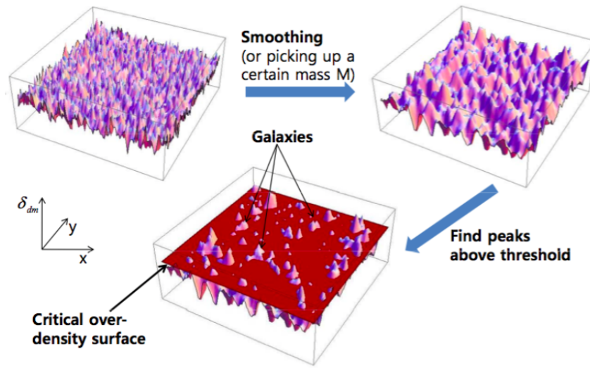
FIGURE 3.7 – Illustration of the peak-bias formalism : peaks above a given threshold in the initial density field correspond to regions where galaxies will form.
