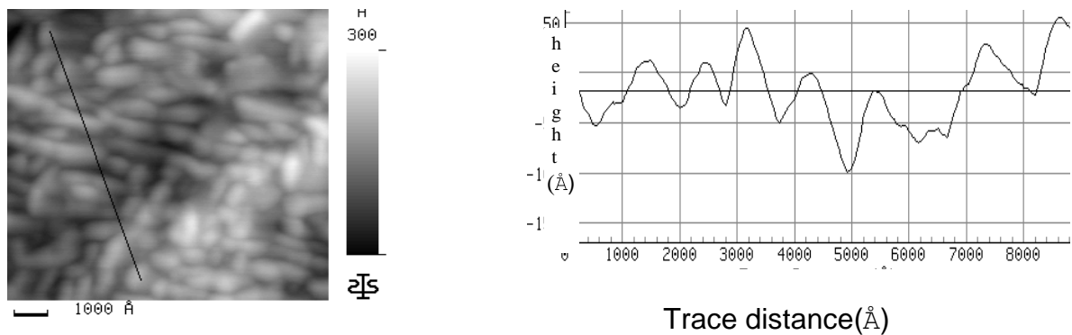
figure n°9 : AFM image and height profile of sample F
