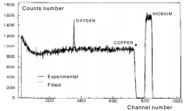
figures n°7 and n°8 : NRS spectrum of sample C annealed at 673 K and sample F sputtered at 673 K
