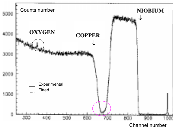
Figure n°4 : RBS spectrum of sample E annealed at 1073 K
