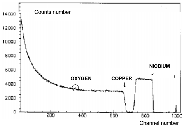
figure n°2 : RBS spectrum of unheated sample B
