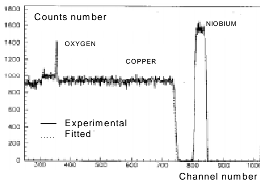
figures n°7 and n°8 : NRS spectrum of sample C annealed at 673 K and sample F sputtered at 673 K
