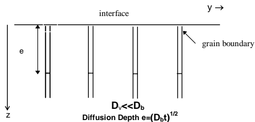
fig n°11 : Schematic Illustration of one type of Diffusion Kinetic (with a model of polycrystal with uniformly spaced grain boundaries)
