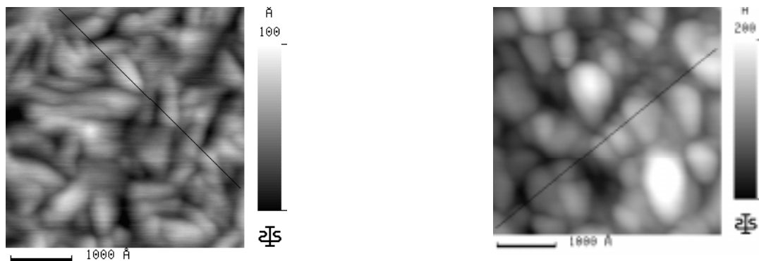
figure n°10 : AFM images of unheated sample ( left ) and sample annealed at 1073K (right)
