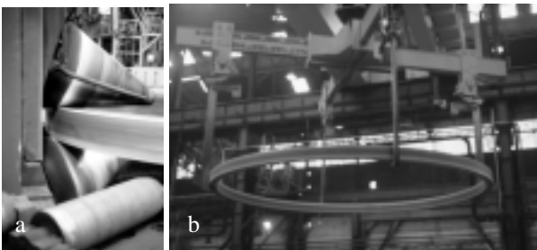
Fig. 2: A 6.8 m diameter ring during two phases of fabrication: seamless ring rolling (a) and transfer of the rolled ring to the quench bath (b).
