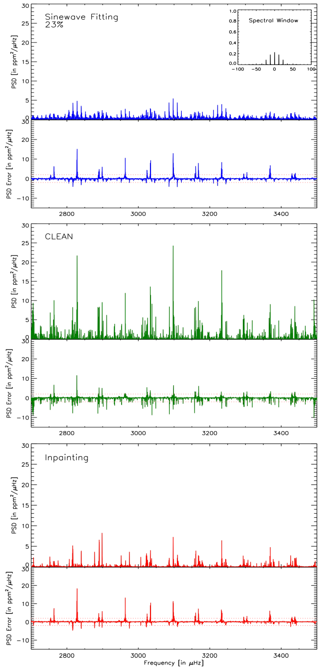
Figure 3. Power Density Spectrum (in units of \text{ppm}^2/\mu\text{Hz} ) for a duty cycle of 23%. The PDS is calculated with a least-squares sinewave fit on the incomplete time series (top panel), using an FFT on the CLEANed time series (middle panel) and using an FFT on the inpainted time series (bottom panel). The errors correspond to the difference between the original PDS and the PDS estimated from the incomplete data. The inset corresponds to the spectral window of the time series.
