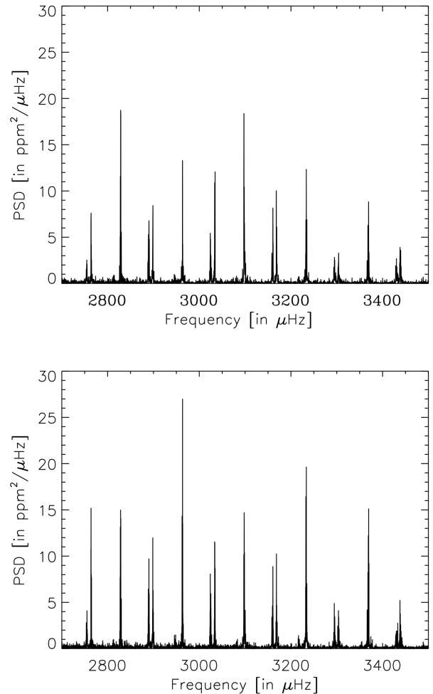
Figure 1. Power Density Spectrum (in units of \text{ppm}^2/\mu\text{Hz} ) of VIRGO/SPM data in the frequency range between 2700 to 3500 \mu\text{Hz} estimated with a Fast Fourier Transform from a complete time series of 50 days (top) and 91.2 days (bottom).
