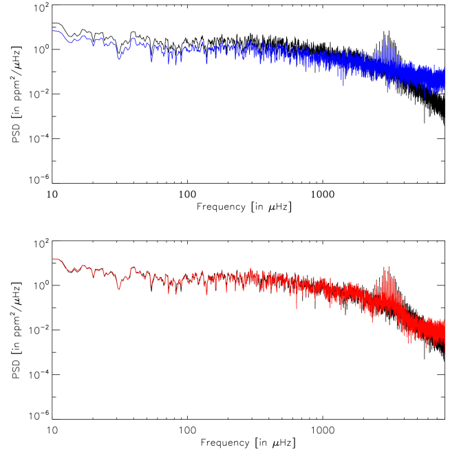
Figure 7. Power Density Spectrum smoothed with a 4 points boxcar function (in units of \text{ppm}^2/\mu\text{Hz} ) estimated from a time series of 24 days of VIRGO/SPM masked with a mask of CoRoT with a duty cycle of 70%. The black curve corresponds to the original PDS estimated from the complete data. In the top panel, the blue curve corresponds to the PDS calculated with a least-squares sinewave fit on the incomplete data. Bottom panel, the red curve correspond to the PDS estimated using a Fast Fourier Transform on the inpainted data.
