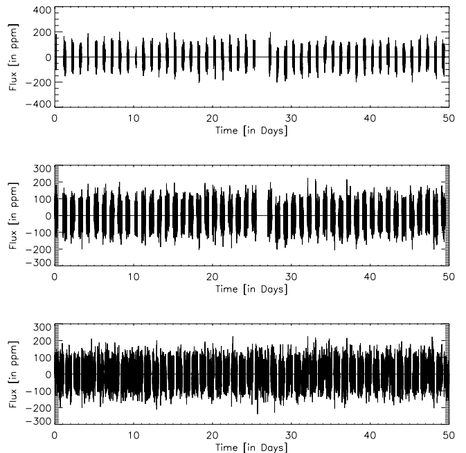
Figure 2. Sample of 50 days of the original VIRGO/SPM data multiplied by a MARK-I like mask to simulate ground-based observations from: a single site corresponding to a duty cycle of 23% (top panel), two different sites with a duty cycle of 50% (middle panel), and from multiple sites corresponding to a duty cycle of 77% (bottom panel).
