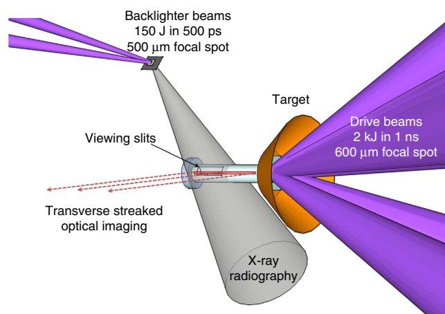
Figure 1 | Schematic of the experimental set-up. The laser beams from the Orion facility are arranged in two cones, which we refer to as ‘drive’ and ‘backlighter’. The drive cone consisted of five beams, which illuminated the target in a 100^\circ cone angle, with each beam supplying \sim 400 J (2 kJ in total) in 1 ns onto a 600- \mu\text{m} spot, which gave an average intensity of 7.0 \times 10^{14} \text{W cm}^{-2} . For the backlighter cone, we used two laser beams of total energy 150 J, in 500 ps onto a 500- \mu\text{m} spot, which gave an average intensity of 1.5 \times 10^{14} \text{W cm}^{-2} . Both sets of beams were delivered at the third harmonic with a wavelength of 351 nm. Viewing slits, along the X-ray diagnostic line of sight, were cut on either side of the tube at the obstacle end.
