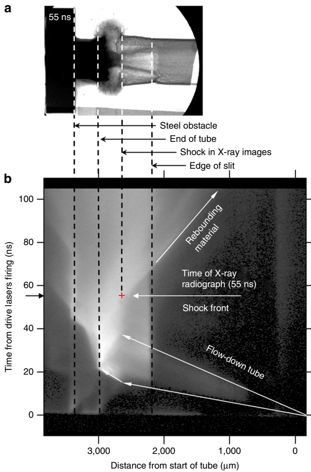
Figure 3 | Streaked optical image of the flow and shock evolution. (a) An X-ray image taken from Fig. 2 aligned with the streaked optical image in (b) . Optical diagnostics were fielded in the experiment to record the self-emission from the hot plasma along the entire length of the tube. An imaging system directed the light emitted by the interacting plasma to the streak camera. The streak camera had a spatial field of view of \sim 4 mm and thus the entire tube and obstacle were visible, except the region shielded by the copper cone. An imaging line aligned with the central axis of the tube (along the slit cut-out in the tube), in the horizontal plane, was then streaked in time over \sim 60 , 100 or 250 ns as required. This provided a temporal dependence of flow velocities in plasma. Time runs from bottom to top, distance right to left. The time evolution of the plasma can clearly be seen inside the tube. The dotted lines and overlaid radiograph show positions of parts of the target on the streaked image. There is good agreement in the position of features between the X-ray (a) and optical (b) diagnostics.
