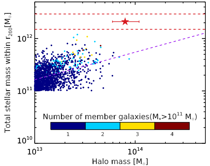
Figure 10. The stellar mass content versus total halo mass for massive halos at z = 2.5 \pm 0.2 from mock catalogs. The total stellar masses are calculated for galaxies with K_s < 23.4 mag and M_* > 10^{11} M_\odot within R_{200c} of the halo center, as defined as the most massive galaxy in each halo. The data point for each halo is color-coded by the number of member galaxies with M_* > 10^{11} M_\odot . The purple dashed line indicates the best linear fit of the stellar mass-to-halo mass relation based on the data points. The stellar mass estimate for CL J1001 and its uncertainties are denoted by the red dashed lines. The red star indicates our estimate of the halo mass and total stellar mass (also only accounting for galaxies with M_* > 10^{11} M_\odot ) for CL J1001.
