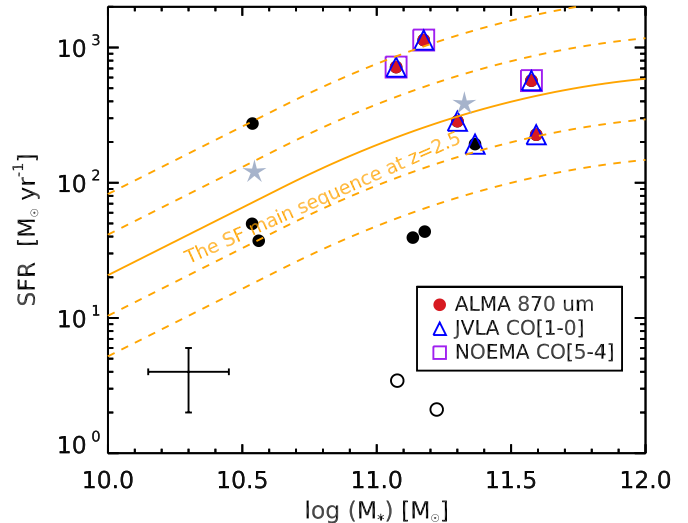
Figure 13. SFR-stellar mass relation for the 13 member galaxies in the cluster core (within 10'' ). Filled circles denote galaxies that are classified as star-forming while open circles are galaxies classified as quiescent based on the rest-frame U - V versus V - J diagram. Galaxies that are detected with S/N > 5 at 870 \mu m with ALMA, CO(1-0) with JVLA and CO(5-4) with IRAM-NOEMA are respectively denoted by red filled circles, blue open triangles and purple open squares. SFRs for ALMA 870 \mu m -detected sources are derived from their infrared luminosity while the others are from SED fitting. The main sequence of field star-forming galaxies at z \sim 2.5 and associated 0.3 dex and 0.6 dex scatter (Schreiber et al. 2015) are shown with orange lines. The filled stars indicate the mean value for the star-forming members in two mass bins separated at M_* = 10^{11} M_{\odot} .
