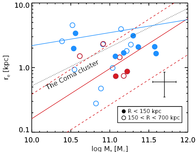
Figure 14. Mass-size relation for quiescent and star-forming candidate members of the structure. Galaxies within R < 150 kpc from the core are denoted by filled circles while those within 150 < R < 700 kpc are denoted by open circles. UVJ -quiescent galaxies are shown in blue while UVJ -star-forming galaxies are shown in red. The mass-size relation for quiescent and star-forming field galaxies at z \sim 2.5 (van der Wel et al. 2014) are shown with red and blue lines, respectively. The 1\sigma scatter of the mass-size relation for field quiescent galaxies is shown with red dashed lines. The large error bar in the bottom-right indicates typical uncertainties of mass and size measurements of our sample galaxies. The mass-size relation for the nearby Coma cluster is indicated with the dotted line (Andreon 1996).
