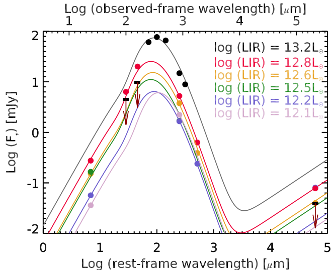
Figure 12. Infrared SEDs for the 5 candidate members with ALMA 870 \mu\text{m} detections. The colored solid lines show the SED-fitting results for the 5 ALMA detections while the black line show the SED-fitting result for the combined flux densities in the core. The 3\sigma upper limits for non-detections at 100 \mu\text{m} , 160 \mu\text{m} , and 1.4 GHz are shown.
