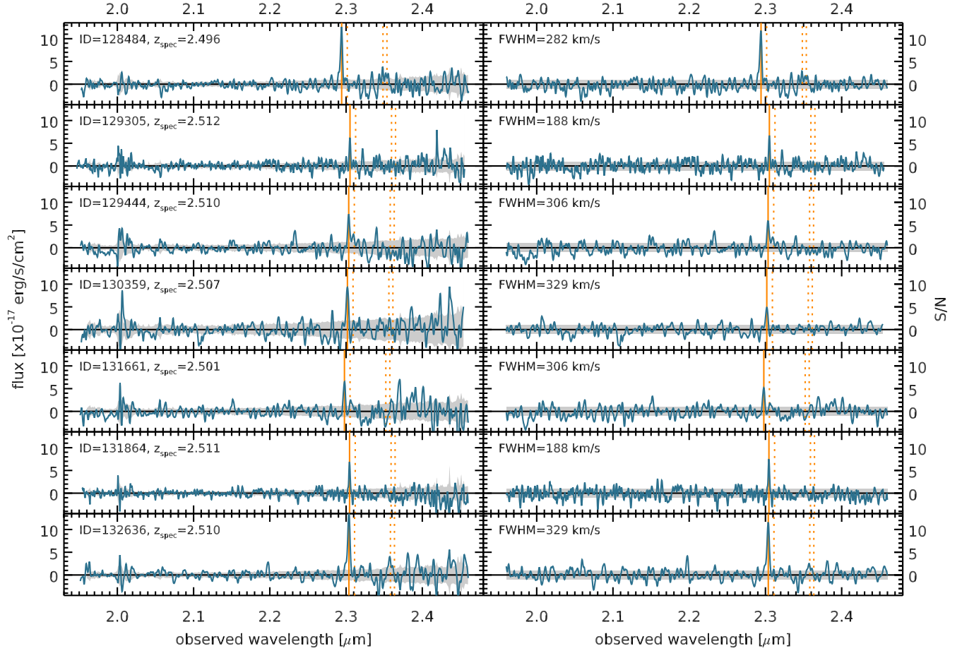
Figure 5. Extracted and smoothed one-dimensional K-band KMOS spectra (left) and the corresponding S/N plot (right) for cluster members. The best-fit FWHM of each H\alpha line is indicated in the right panels, which was used to smooth the spectra. All the listed sources are detected with a S/N > 5 except source 130359, which is detected at 4.9\sigma . Though in most cases we have only detected one line, given the range of their photometric redshifts (Table. 1) we determined their redshifts assuming the line to be H\alpha . The position of the H\alpha line is indicated by the solid line while dotted lines show the expected position of [NII] as well as the [SII] doublet.
