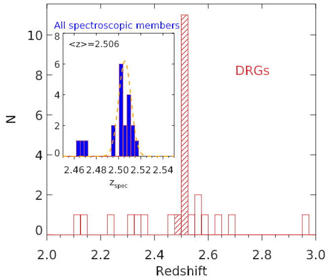
Figure 7. Redshift distributions of the galaxies in and around the overdensity. The histogram in red shows the redshift distribution for all DRGs within 2' from the core of the structure. DRGs with spectroscopic redshift are indicated by the line-filled histogram. The inner panel shows the redshift distribution of all the galaxies in and around the overdensity (including non-DRGs) with spectroscopic redshift 2.45 < z_{\text{spec}} < 2.55 from our spectroscopic surveys.
