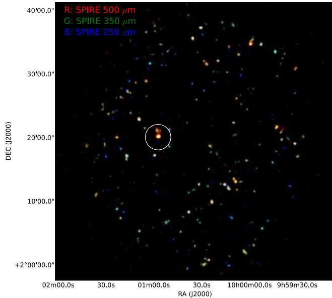
Figure 2. RGB Herschel/SPIRE composite color image of the COSMOS field covered by the CANDELS-Herschel survey. The R , G and B channel correspond to SPIRE 500, 350 and 250 \mu\text{m} , respectively. Only sources brighter than 20 mJy at least at one of the three SPIRE wavelengths are shown. Sources with redder colors tend to be at higher redshifts. The large white circle with a radius of 2' indicates the position of the galaxy overdensity, which is the brightest SPIRE source in the whole field.
