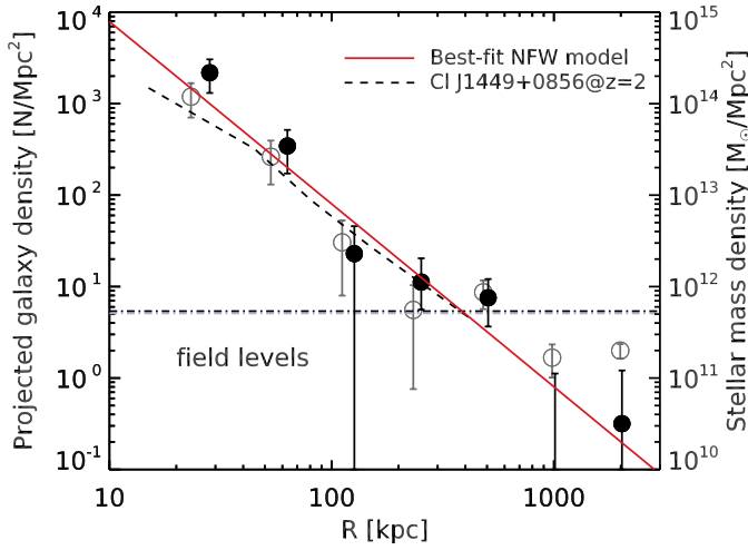
Figure 9. The projected number (open circles) and mass densities (filled circles) of DRGs extending to \sim 2 Mpc from the overdensity. The average number and mass densities of field DRGs, as denoted by the grey and black horizontal line, have been subtracted from the data points. The best-fitting projected NFW profile, which has a scale radius R_s = 0_{-0}^{+8} kpc, is shown by the red line. The stellar mass density profile of the mature X-ray cluster Cl J1449+0856 at z = 2 (Gobat et al. 2011; Strazzullo et al. 2013) is shown as the dashed line.
