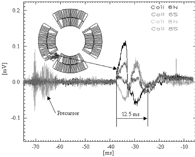
Fig. 2. Quench antenna analysis : these are the voltage drop measured on the four pick-up coils of a quench antenna during Quench number one. The inset shows the resulting quench localization.
