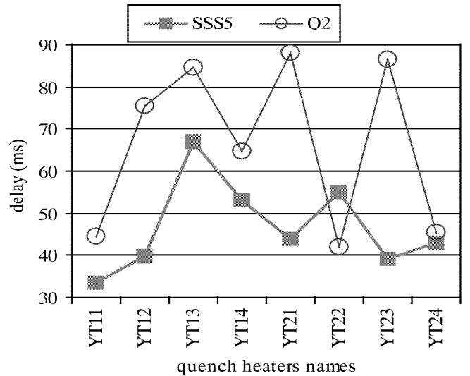
Fig. 4. Delay for quenches at 10kA provoked by a single quench heater. Q2 is a previous design quadrupole and SSS5 is the new design.
