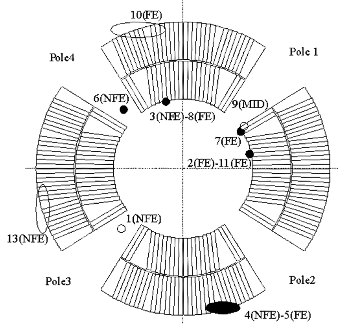
Fig. 3. Quench localization : ● - Quench in aperture one, ○ - Quench in aperture two. (FE) means a quench in Feed-End, (NFE) quench in Non Feed-End, and (MID) in the middle of the straight part.
