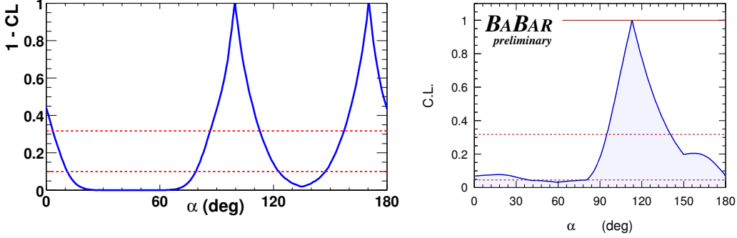
Figure 1: Confidence level on \alpha for B \rightarrow \rho\rho analysis (right plot) and for B^0 \rightarrow \pi^+ \pi^- \pi^0 analysis (left plot). The dashed lines correspond to the 68% (top) and 90% (bottom) CL intervals.
