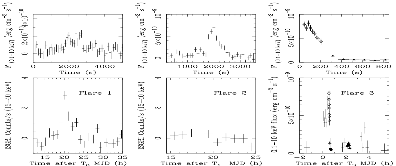
FIG. 1.— Bottom, from left: IBIS/ISGRI (flare 1,2) and Swift (flare 3) light curves. IBIS data are binned at \sim 2 ks. In the last panel the crosses represent the extrapolated BAT flux, while the diamonds and triangles the XRT/WT and PC data. The time axis is expressed in hours after T_0=52821.0 , T_1=53870.0 , and T_3=54012.615 MJD, respectively. The Swift light curve shows also weak flares e.g. at t\sim 3.5 h IGR J08408–4503 is detected in BAT at \sim 7\sigma level. Top: the brightest part of each outburst is shown on a smaller time scale (100 s time bin for ISGRI).
