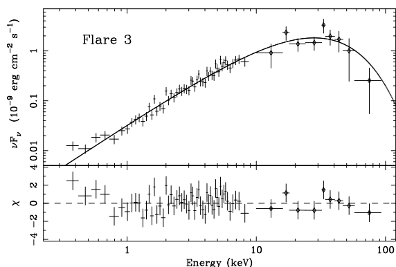
FIG. 2.— Combined XRT (crosses) and BAT (diamonds) spectra of flare 3. The best fit PL high energy cut-off model and the residuals (lower panel) are shown.
