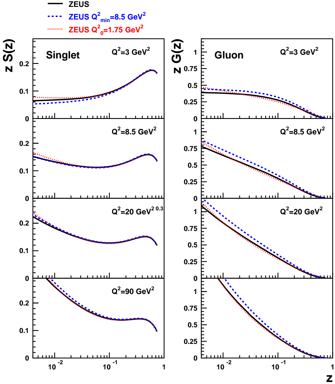
FIG. 15. Singlet and gluon distributions of the Pomeron as a function of z derived from QCD fits on ZEUS data. Results are presented with Q_{\min}^2 = 4.5 \text{ GeV}^2 (full lines), Q_{\min}^2 = 8.5 \text{ GeV}^2 (dashed lines). Distributions obtained from a fit with Q_0^2 = 1.75 \text{ GeV}^2 (dotted lines) is also shown.
