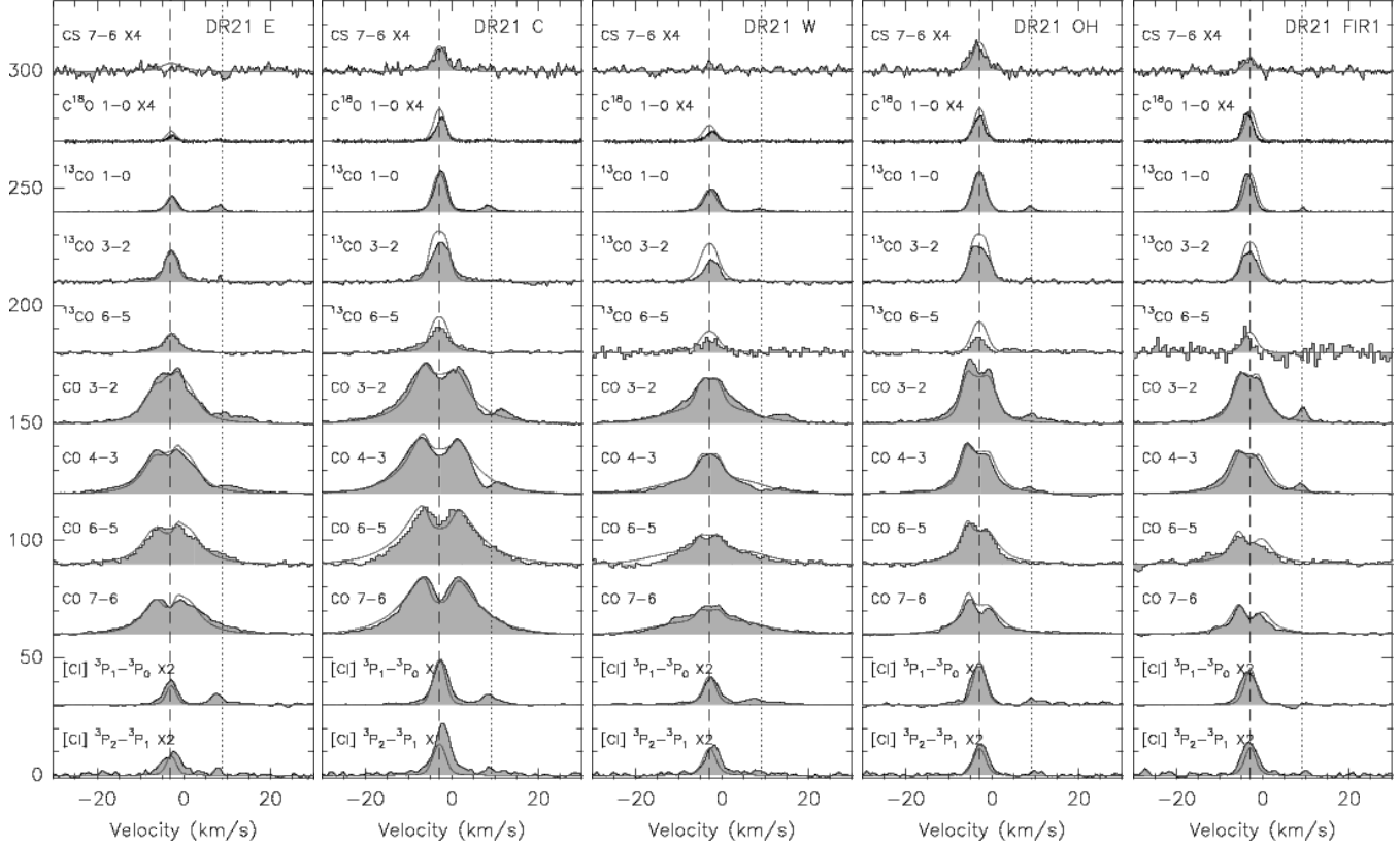
Fig. 5. Spectra of all observed species at the five ISO positions. Grey filled spectra outlined in black: observed lines, thin grey lines: line profiles modeled with the radiative transfer code SIMLINE (see Sect. 4.2). All spectra are shown at a common spatial resolution of 80'' and on a T_{\text{mb}} scale. The baselines are shifted in steps of 30 K. [C I] was multiplied by a factor of 2, CS 7–6 and \text{C}^{18}\text{O} 1–0 by a factor of 4. J = 1-0 transition data are FCRAO observations. The dashed lines indicate the central velocity of -3 \text{ km s}^{-1} , and the dotted lines the secondary velocity component at about 9 \text{ km s}^{-1} , which was excluded from the fitting.
