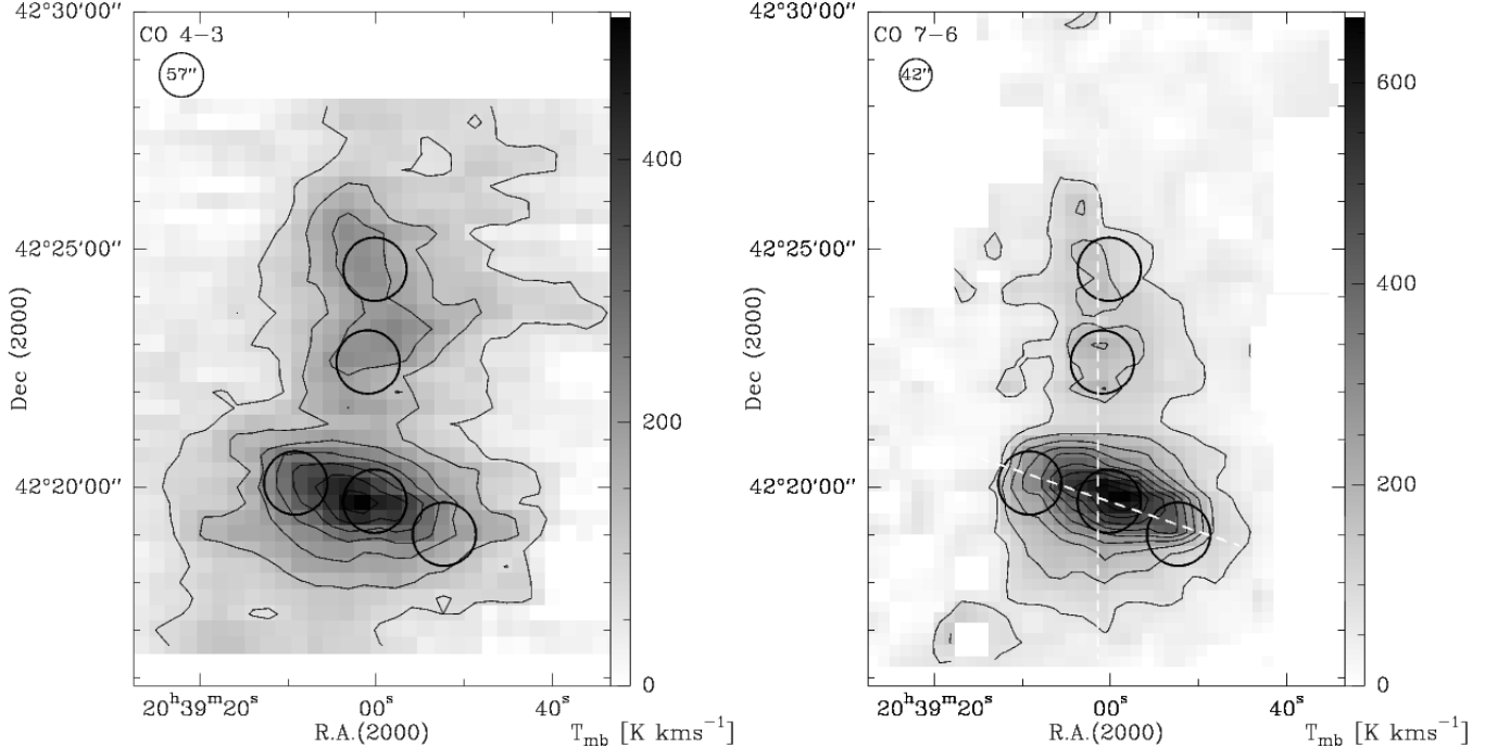
Fig. 2. Integrated intensity map of CO 4–3 ( left ) and CO 7–6 ( right ) of DR 21 & DR 21 (OH). The integration interval is -20 to 30 \text{km s}^{-1} . The contours for CO 4–3 run from 66(3\sigma) to 462 \text{K km s}^{-1} in steps of 3\sigma , and from 68(2\sigma) to 671 \text{K km s}^{-1} in steps of 2\sigma for CO 7–6. The HPBW is indicated in the upper left corner. The positions of ISO/LWS observations (cf. Fig. 1) are indicated by circles. The dashed white lines correspond to the cuts shown in Fig. 6.
