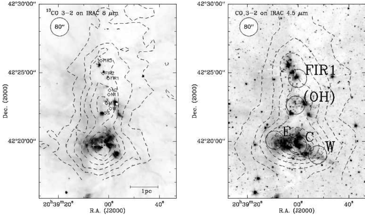
Fig. 1. View of the DR21/DR21(OH) high mass star forming region. Left: Overlay of the KOSMA ^{13}\text{CO} 3–2 map (cf. Schneider et al. (2006)/SBS2006) in contours on a Spitzer IRAC 8\ \mu\text{m} greyscale map (Marston et al. 2004). Contours are on a T_{\text{mb}} scale and range from 16.8 to 100.8 in steps of 16.8\ \text{K km s}^{-1} ( \sigma = 5.6\ \text{K km s}^{-1} ). The integration interval is -10 to 20\ \text{km s}^{-1} . The left-top circle indicates the HPBW of KOSMA. The map also shows 6 positions of radio continuum sources identified as OB stars by Roelfsema et al. (1989) (white crosses), 2 infrared sources and maser positions (Garden et al. 1986) (small white circles), and 8 compact 1.3-mm dust emission sources (Chandler et al. 1993) (open rectangles). Right: Overlay of the Spitzer map at 4.5\ \mu\text{m} with contours of the KOSMA ^{12}\text{CO} 3–2 map (integration interval of -20 to 30\ \text{km s}^{-1} ; discussed in SBS2006) ranging from 18 to 450 in steps of 48\ \text{K km s}^{-1} ( \sigma = 6\ \text{K km s}^{-1} ). The labeled circles mark the positions and beam sizes of the ISO/LWS observations that we use to constrain the physical parameters as discussed in the text. The LWS beam is comparable to the resolution of the KOSMA maps.
