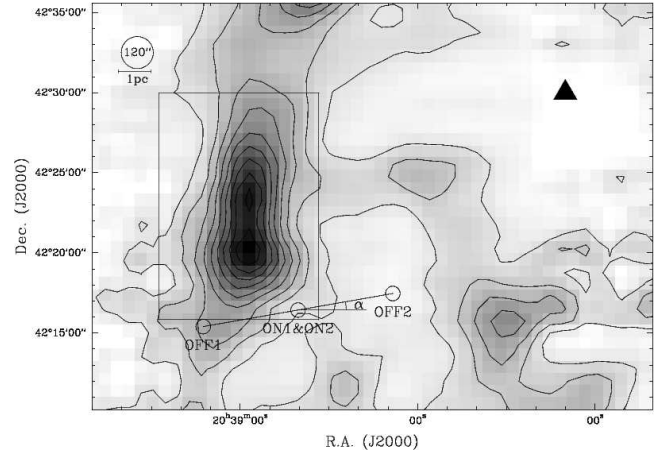
Fig. B.1. On-The-Fly map of the ^{13}\text{CO} 2–1 emission (SBS2006). An emission-free position is indicated by the triangle on the right and was used as OFF position for the OTF observations. The box indicates the map size of DBS observations in Fig. 2 and 3. The circle in the top left corner indicates the 120'' beam size. The smaller circles labeled ON1&ON2, OFF1, and OFF2 show an exemplary DBS measurement (cf. Fig. B.2) with a field rotation angle \alpha = 10^\circ .
