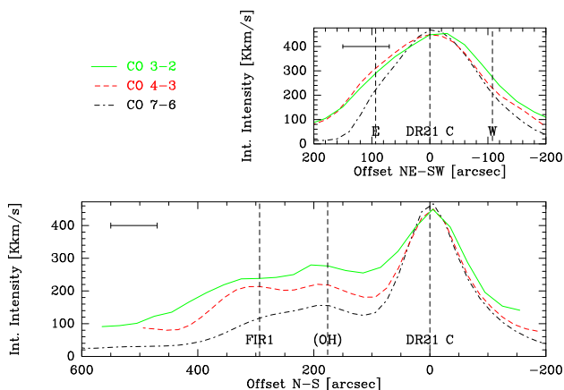
Fig. 6. Cut along the DR21 outflow axis ( top ) and along the ridge ( bottom ) centered on DR21 C in CO 3–2, 4–3, and 7–6 integrated emission. The 80'' resolution is indicated as horizontal line. The dashed vertical lines indicate the positions of the ISO/LWS observations.
