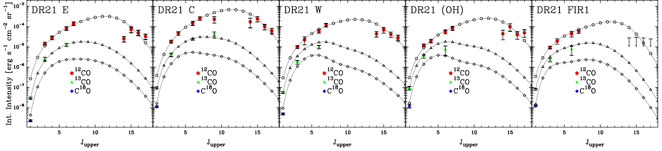
Fig. 8. Cooling curves of the best-fit model line fluxes (marked by open symbols) of CO, ^{13}\text{CO} , and \text{C}^{18}\text{O} . Observed line intensities are indicated as filled symbols (see Table 3). At position DR21 C, we included two observations by Boreiko & Betz (1991) of CO and ^{13}\text{CO} J = 9-8 . Since the ^{13}\text{CO} 6–5 map does not cover the positions DR21 (OH) and DR21 FIR1 on a fully sampled grid, we expect a larger error. The high- J CO emission at DR21 FIR1 are upper limits.
