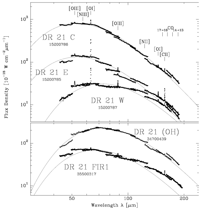
Fig. 7. ISO/LWS Spectral Energy Distribution (SED) of the DR 21 region ( upper panel ), and the DR21 (OH) and DR21 FIR1 region ( lower panel ). Curves indicate the best greybody fit corresponding to the values given in Table 5.
