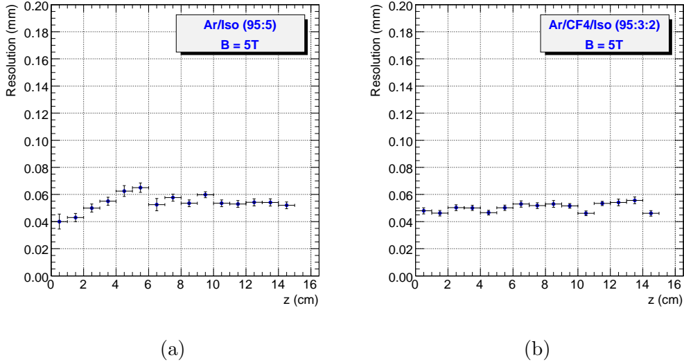
Fig. 3. Transverse resolution as a function of drift distance for 2 mm x 6 mm pads for a magnetic field of 5 T for two gases mixtures: (a) Ar:iC 4 H 10 /95:5 and (b) Ar:CF 4 :iC 4 H 10 /95:3:2.
