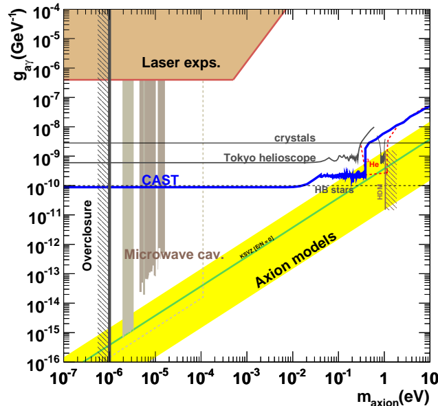
Figure 1: Exclusion plot in the axion-photon coupling versus the axion mass plane for a wide range of parameters. The limit achieved by the CAST experiment (combined result of the CAST phase I and ^4\text{He} part of phase II) is compared with constraints obtained from the Sumico experiment (the Tokyo helioscope) and HB stars. The red dashed line shows our prospects for the ^3\text{He} run started in March 2008. The vertical line (HDM) is the hot dark matter limit for hadronic axions m_a < 1.0\text{ eV} inferred from observations of the cosmological large-scale structure. The yellow band represents typical theoretical models with |E/N - 1.95| in the range 0.07–7 where the green solid line corresponds to the case when E/N = 0 is assumed. Limits from laser, microwave and underground detectors [18] for axion searches have been included.
