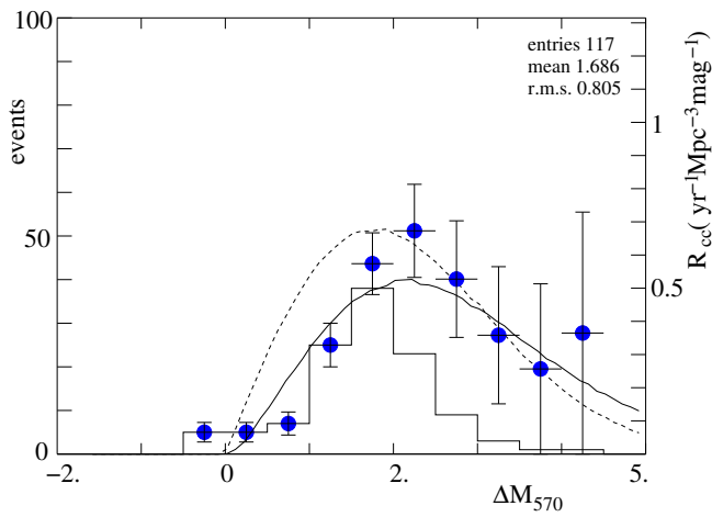
Fig. 12. The differential SNcc rate. The data points are those of Figure 11 with the SNIa subtracted (statistical errors only). The left-hand scale is the number of events and the right-hand scale is the absolute differential rate derived from the total rate in Section 5. The dashed curve shows the intrinsic distribution for a toy model (of no physical motivation) with rate \propto \Delta M_{570} \exp[-(\Delta M_{570}/2.5)^2] while the solid line shows the distribution for this model after including the host absorption predicted by the model of Hatano et al. (1998).
