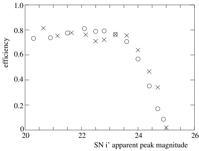
Fig. 5. Pre-selection efficiency as a function of i' . The “efficiency” is defined as the number of reconstructed events in a given magnitude interval divided by the number of generated events in the same interval. The circles are for SNIa and the crosses for SNcc with \tau_{fall} = 100 days.
