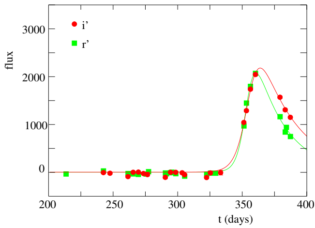
Fig. 1. The r' and i' light curves of a SNIa. The spectroscopic redshift is 0.332, the host photometric redshift 0.294, and the peak magnitude i' = 21.6 . The time corresponds to MJD-52640.
