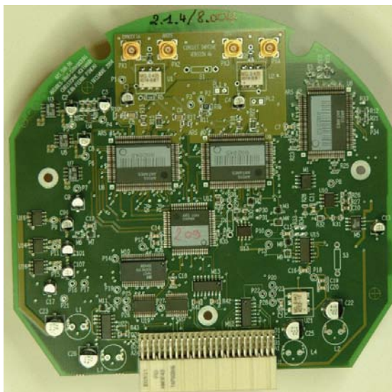
Figure 1. The ARS motherboard (diameter ~15 cm).
