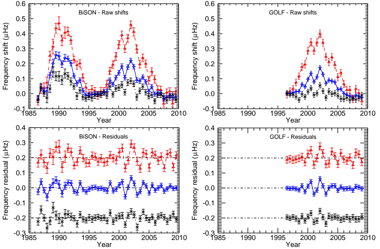
Fig. 1.— Top: average frequency shifts of “Sun-as-a-star” modes with frequencies between 1.88 and 3.71 mHz (total-frequency band, blue solid line and diamond symbols); 1.88 and 2.77 mHz (low-frequency band, black dotted line and cross symbols); and 2.82 and 3.71 mHz (high - frequency band, red dashed line and triangle symbols). Bottom: residuals left after dominant 11-year signal has been removed (black dotted and red dashed curves are displaced by -0.2 and +0.2 , respectively, for clarity).
