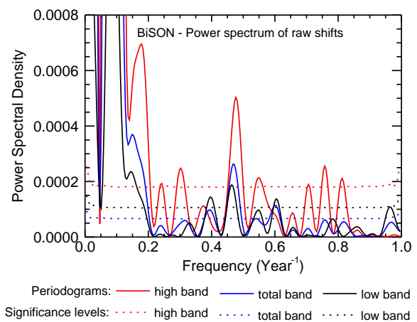
Fig. 2.— Periodograms of the BiSON frequency shifts. The solid lines represent the periodograms of the different frequency bands (see legend). The dotted lines represent the 1 per cent “false alarm” significance levels for the respective frequency ranges.
