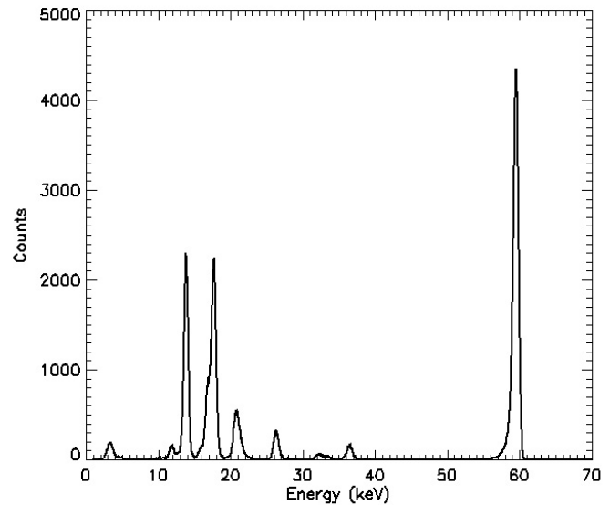
Fig. 13. Sum spectrum with Caliste 64 at -10^{\circ}\text{C} , -400\text{V} , with a ^{241}\text{Am} source and a peaking time of 9.6\text{ }\mu\text{s} . Only the single events are considered. All the pixels contribute to the sum. Energy resolution is 701\text{ eV FWHM} at 13.9\text{ keV} and 805\text{ eV FWHM} at 59.54\text{ keV} . Peak to valley ratio between 59.54\text{ keV} peak and 57\text{ keV} is 100.
