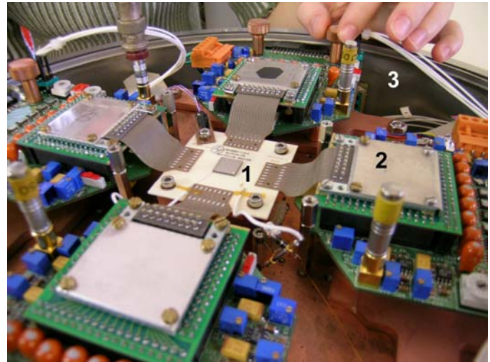
Fig. 4: Set-up of the spectroscopic measurement bench equipped with a 64-pixel CdTe detector prototype. (1) the detector mounted on a flat substrate, (2) a 16-analogue channel IDeF-X V1.0 to read out a quarter of the matrix, (3) the thermal enclosure.
