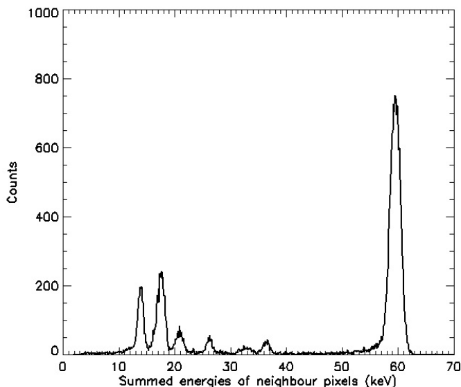
Fig. 15. Spectrum built by adding the energies of all the neighbor pixels that triggered at the same time. Even in case of charge sharing, we can find the energy of incident photon.
