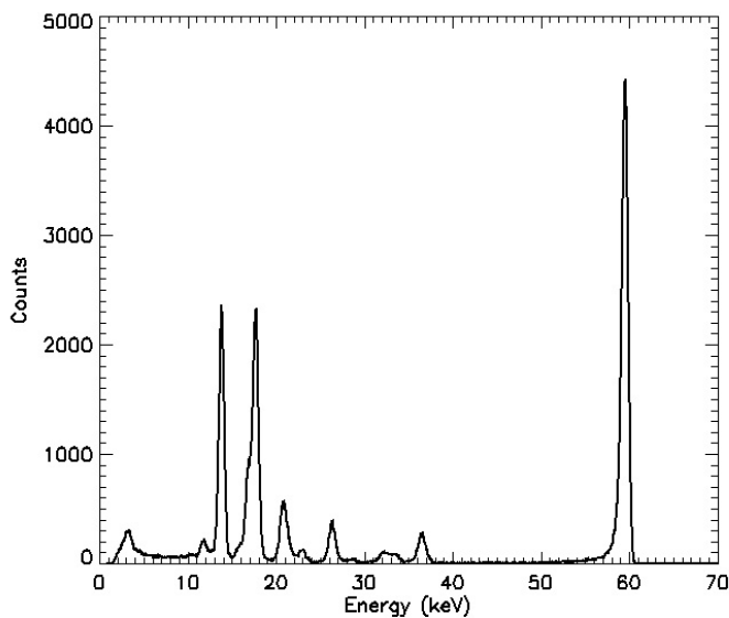
Fig. 12. Sum spectrum with Caliste 64 at -10^{\circ}\text{C} , -400\text{V} , with a ^{241}\text{Am} source and a peaking time of 9.6\text{ }\mu\text{s} . All the pixels contribute to the sum. Energy resolution is 697\text{ eV FWHM} at 13.9\text{ keV} and 808\text{ eV FWHM} at 59.54\text{ keV} . Peak to valley ratio between 59.54\text{ keV} peak and 57\text{ keV} is 62.
