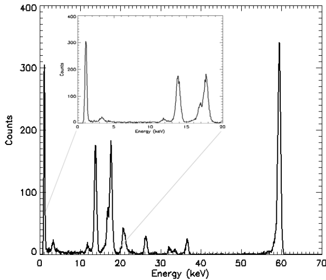
Fig. 11. Spectrum of pixel #1, for a detector cooled to -10^{\circ}\text{C} and biased at -400\text{ V} . Energy resolution is 650\text{ eV FWHM} at 13.9\text{ keV} and 796\text{ eV FWHM} at 59.54\text{ keV} . Multiple lines are visible on the left of the 17.75\text{ keV} peak. The 3.3\text{ keV} line is a source photon whereas the 1.2\text{ keV} structure corresponds to the noise rise and gives information about the low threshold of this pixel.
