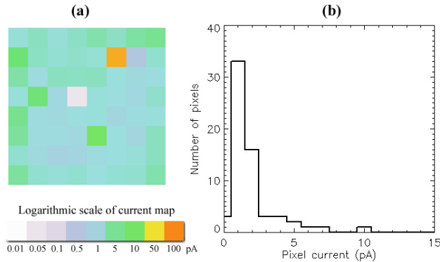
Fig. 3: Results of current measurement with a 1 mm-thick CdTe sample, at -17^{\circ}\text{C} , -400\text{V} . (a) Current map and its logarithmic scale in pA. (b) Histogram of currents. Half of the array has a pixel current between 1 and 2 pA.
