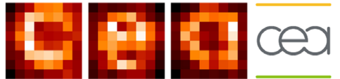
Fig. 8. Three images with Caliste 64, biased at -100V at room temperature. The energy range is centered on 60 keV ^{241}\text{Am} line. Images were taken in one minute. Dark pixels saw about 20 photons whereas bright pixels saw about 200 photons.
