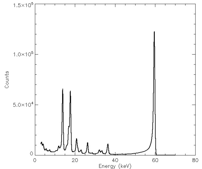
Fig. 5: Sum spectrum of an Al-Ti-Au Schottky CdTe detectors, with 63 out of 64 pixels, at -36^{\circ}\text{C} , -400\text{V} . Energy resolution is 579\text{ eV} FWHM at 13.9\text{ keV} and 767\text{ eV} FWHM at 59.54\text{ keV} . The peak to valley ratio between 59.54\text{ keV} and 57\text{ keV} is 14.8.
