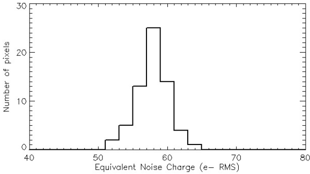
Fig. 6. Histogram of ENC for the 64 pixels of a Caliste 64 electrical body, at 9.6 \mu\text{s} , with a leakage current of about 3 pA.
